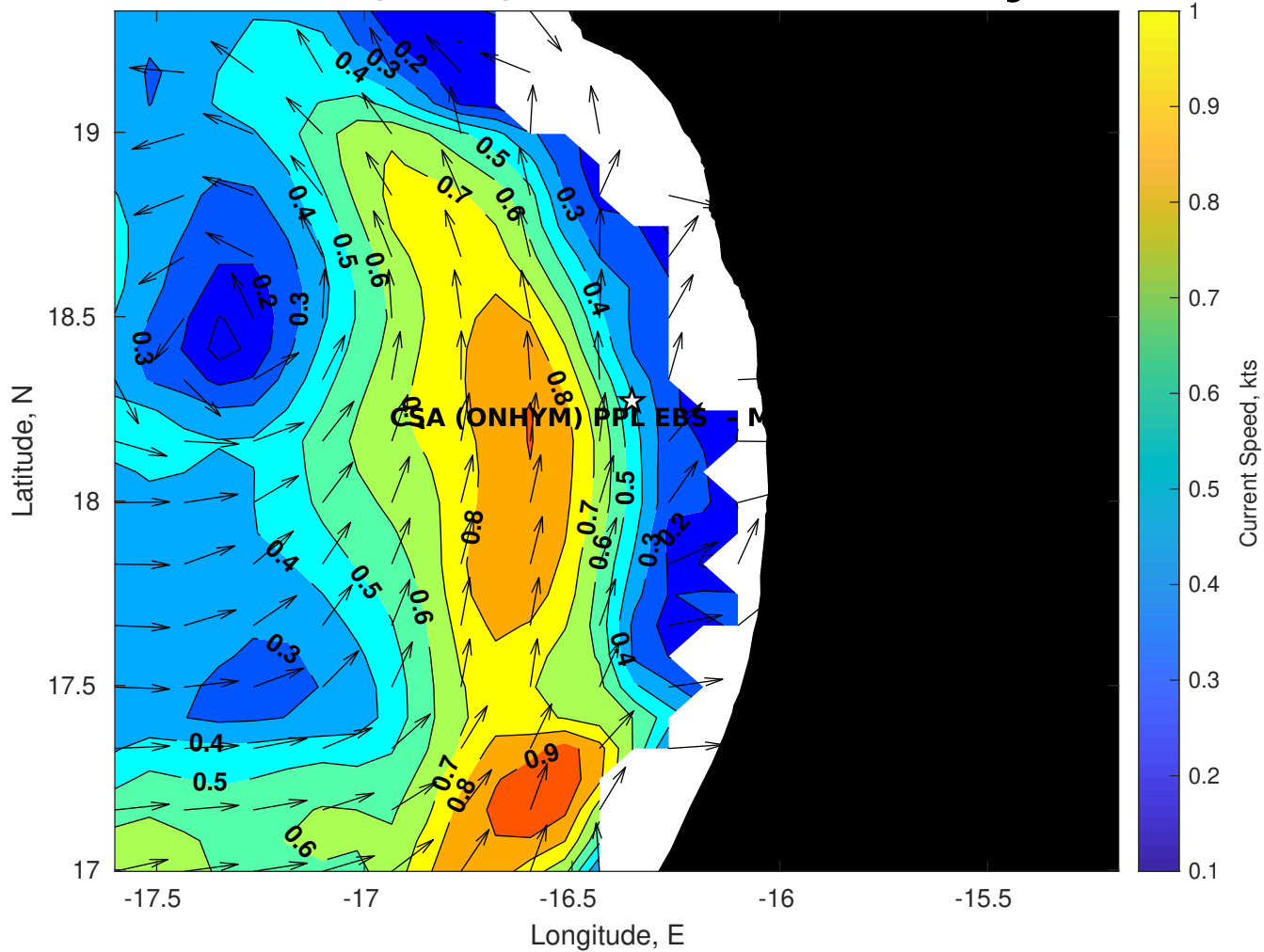
Surface Currents for CSA (ONHYM) PPL EBS - Mauritania at 20-Aug-2025 00:00:00
