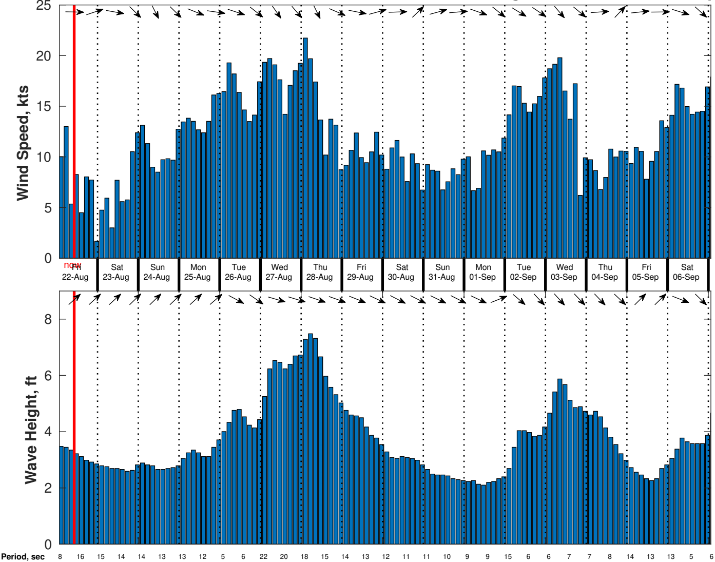
Wind & Wave Forecast for CSA (ONHYM) PPL EBS - Mauritania from 21-Aug-2025 01:00:00 to 06-Sep-2025 01:00:00
