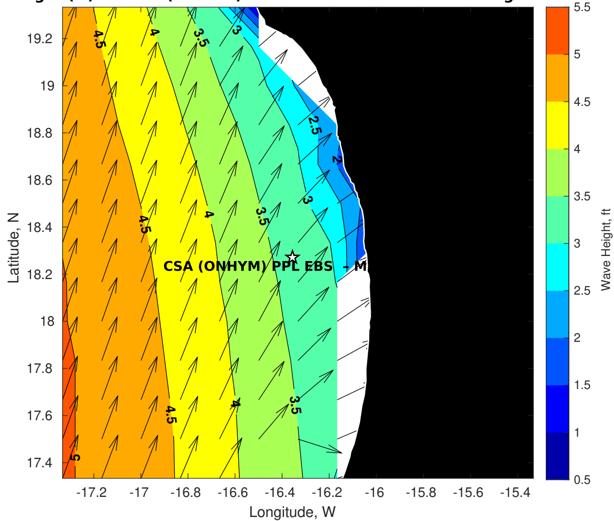
Wave Height (ft) for CSA (ONHYM) PPL EBS - Mauritania at 21-Aug-2025 09:00:00
