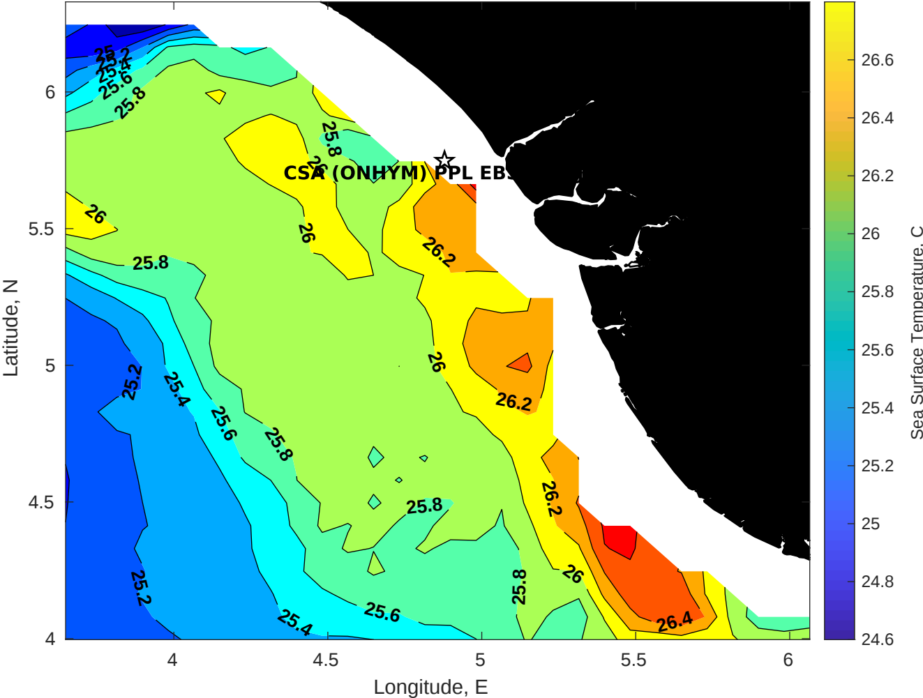
SST for CSA (ONHYM) PPL EBS - Nigeria at 20-Aug-2025 00:00:00
