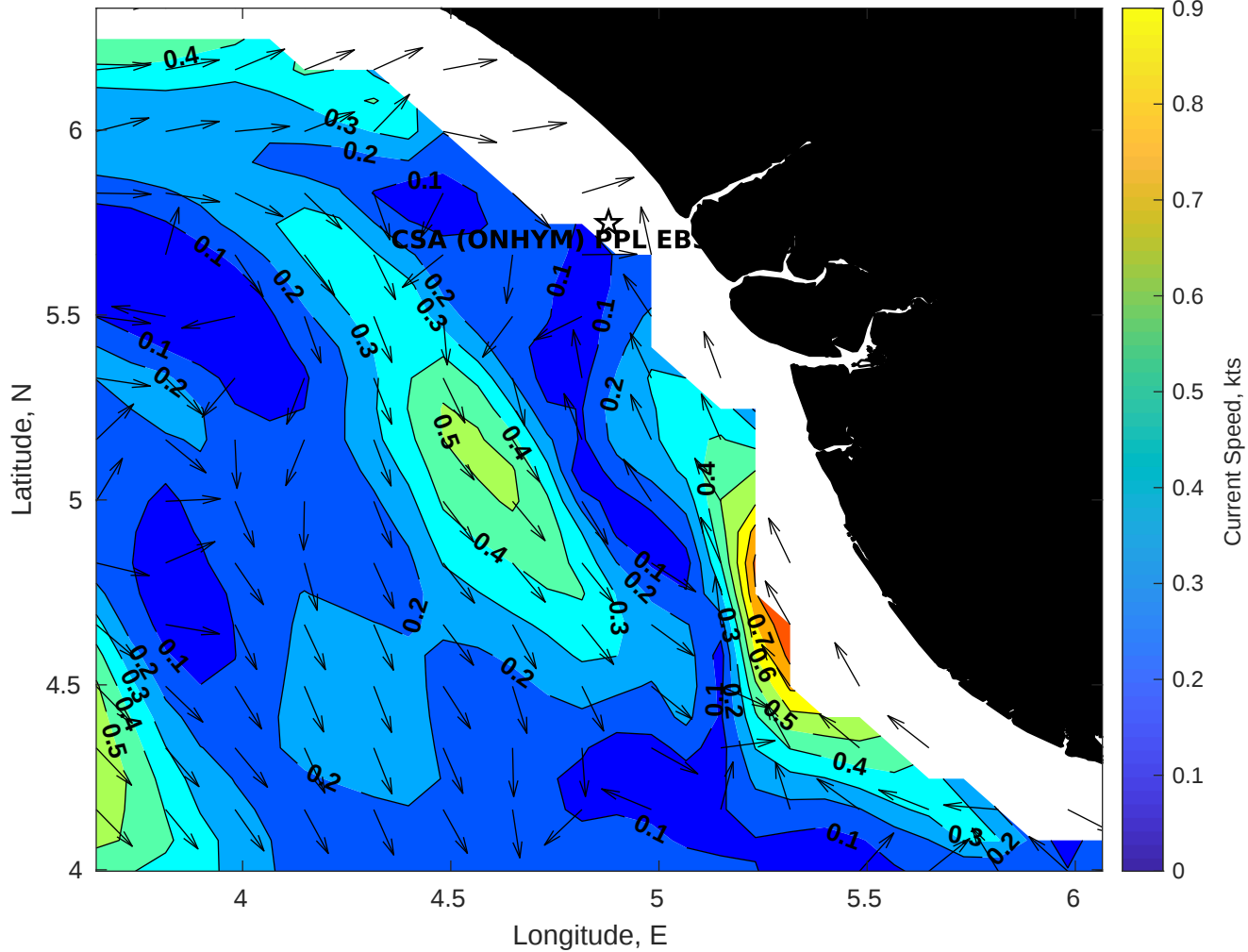
Surface Currents for CSA (ONHYM) PPL EBS - Nigeria at 20-Aug-2025 00:00:00
