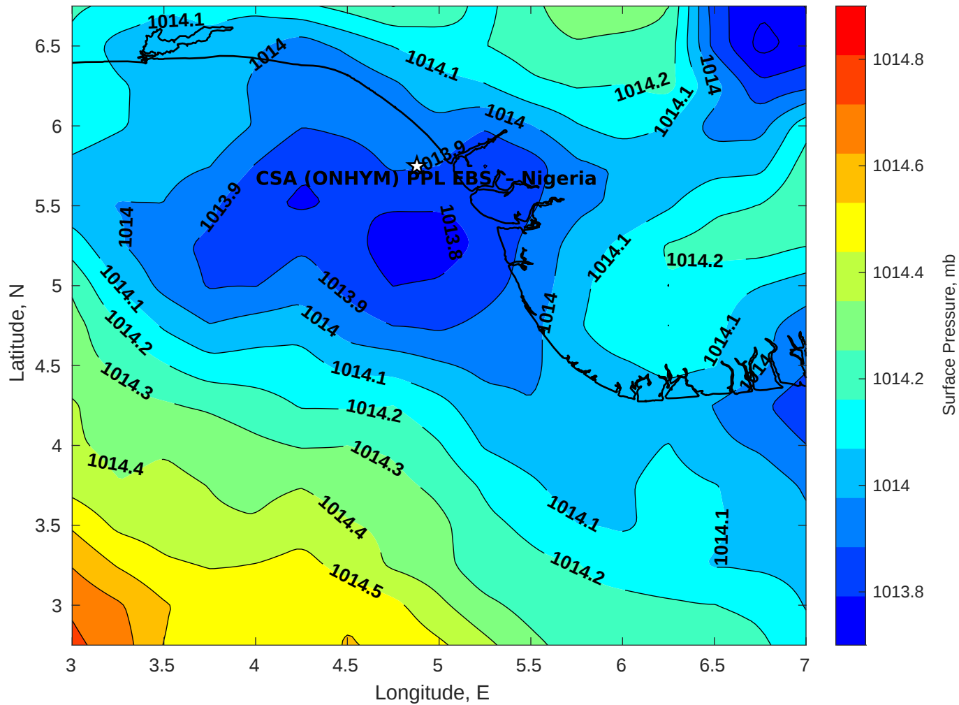
Surface Pressure (mb) for CSA (ONHYM) PPL EBS - Nigeria at 21-Aug-2025 00:00:00
