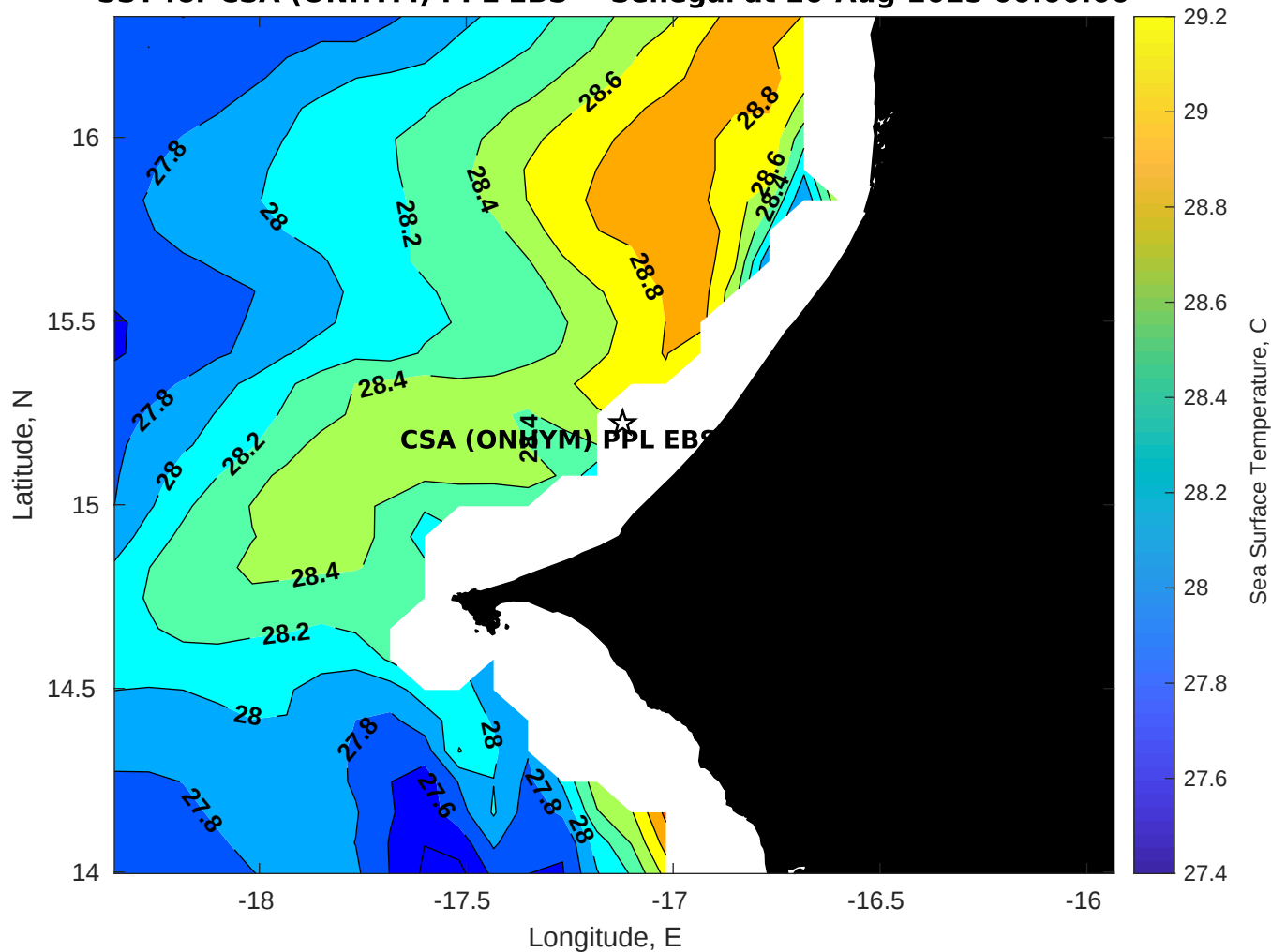
SST for CSA (ONHYM) PPL EBS - Senegal at 20-Aug-2025 00:00:00
