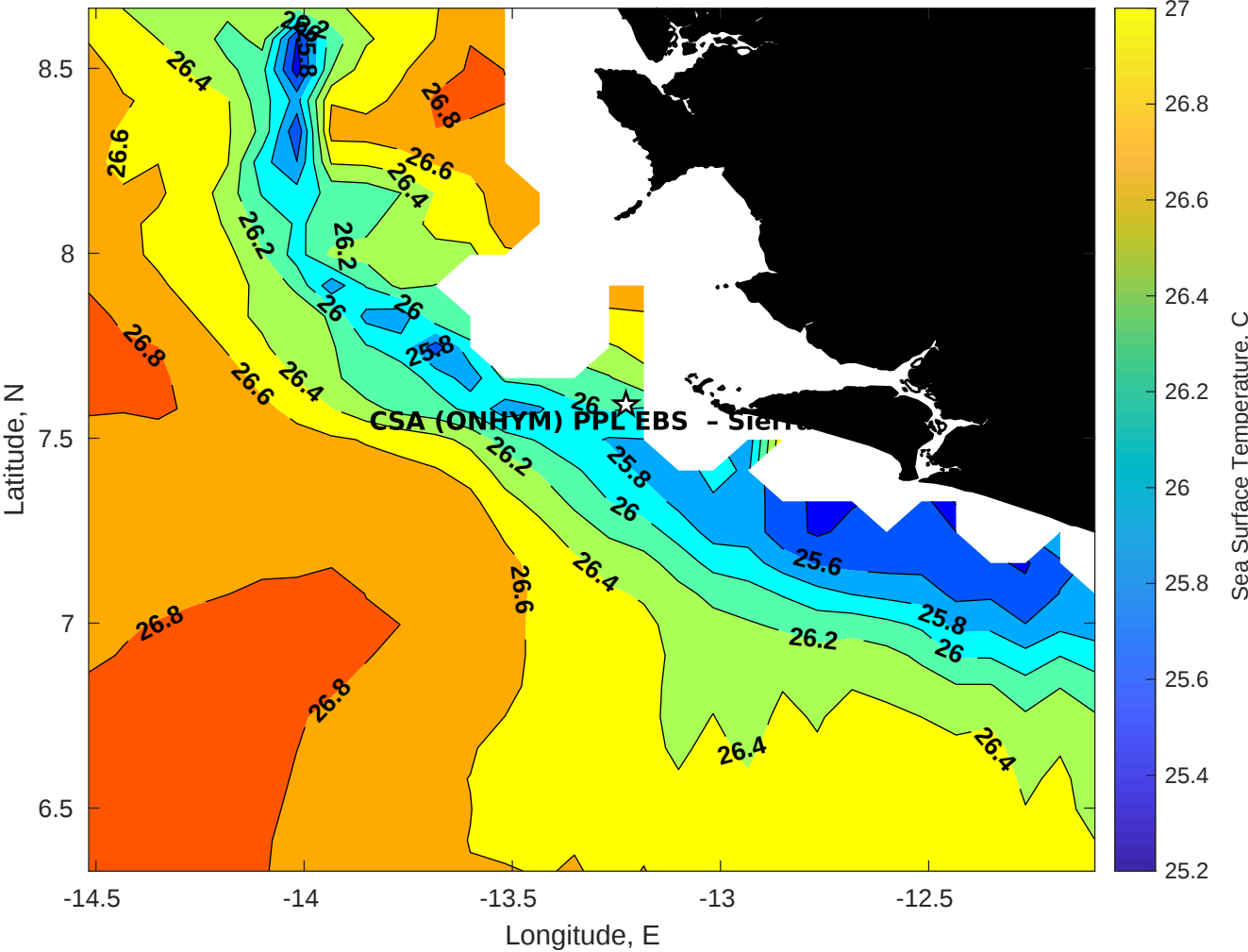
SST for CSA (ONHYM) PPL EBS - Sierra Leone at 20-Aug-2025 00:00:00
