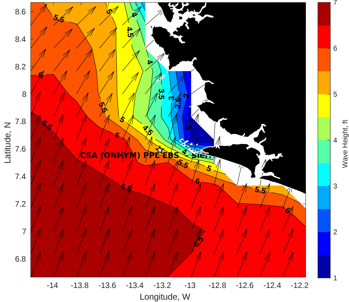
Wave Height (ft) for CSA (ONHYM) PPL EBS - Sierra Leone at 21-Aug-2025 09:00:00
