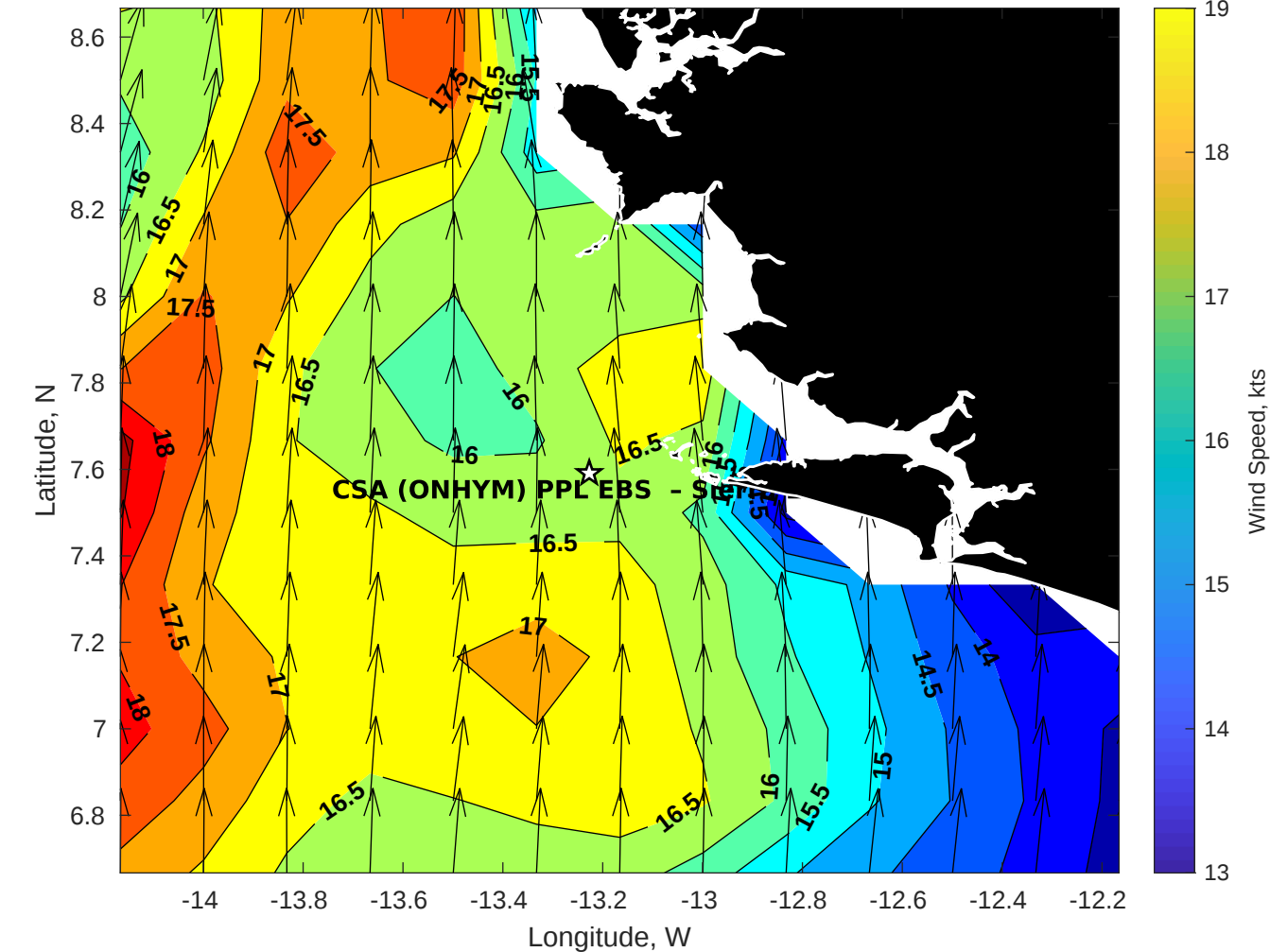
Winds (kts) for CSA (ONHYM) PPL EBS - Sierra Leone at 21-Aug-2025 09:00:00
