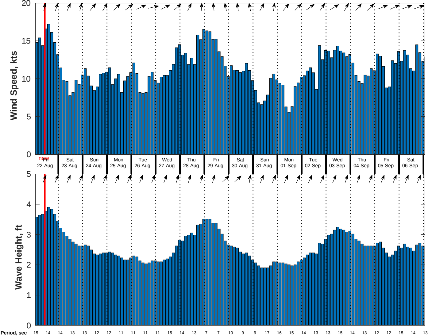
Wind & Wave Forecast for CSA (ONHYM) PPL EBS - Sierra Leone from 21-Aug-2025 01:00:00 to 06-Sep-2025 01:00:00
