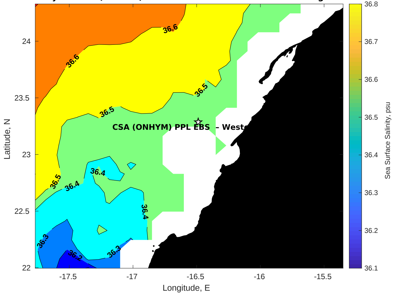
Surface Salinity for CSA (ONHYM) PPL EBS - Western Sahara at 20-Aug-2025 00:00:00
