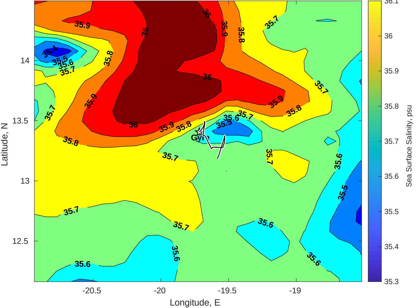
Surface Salinity for Gyre at 20-Aug-2025 00:00:00
