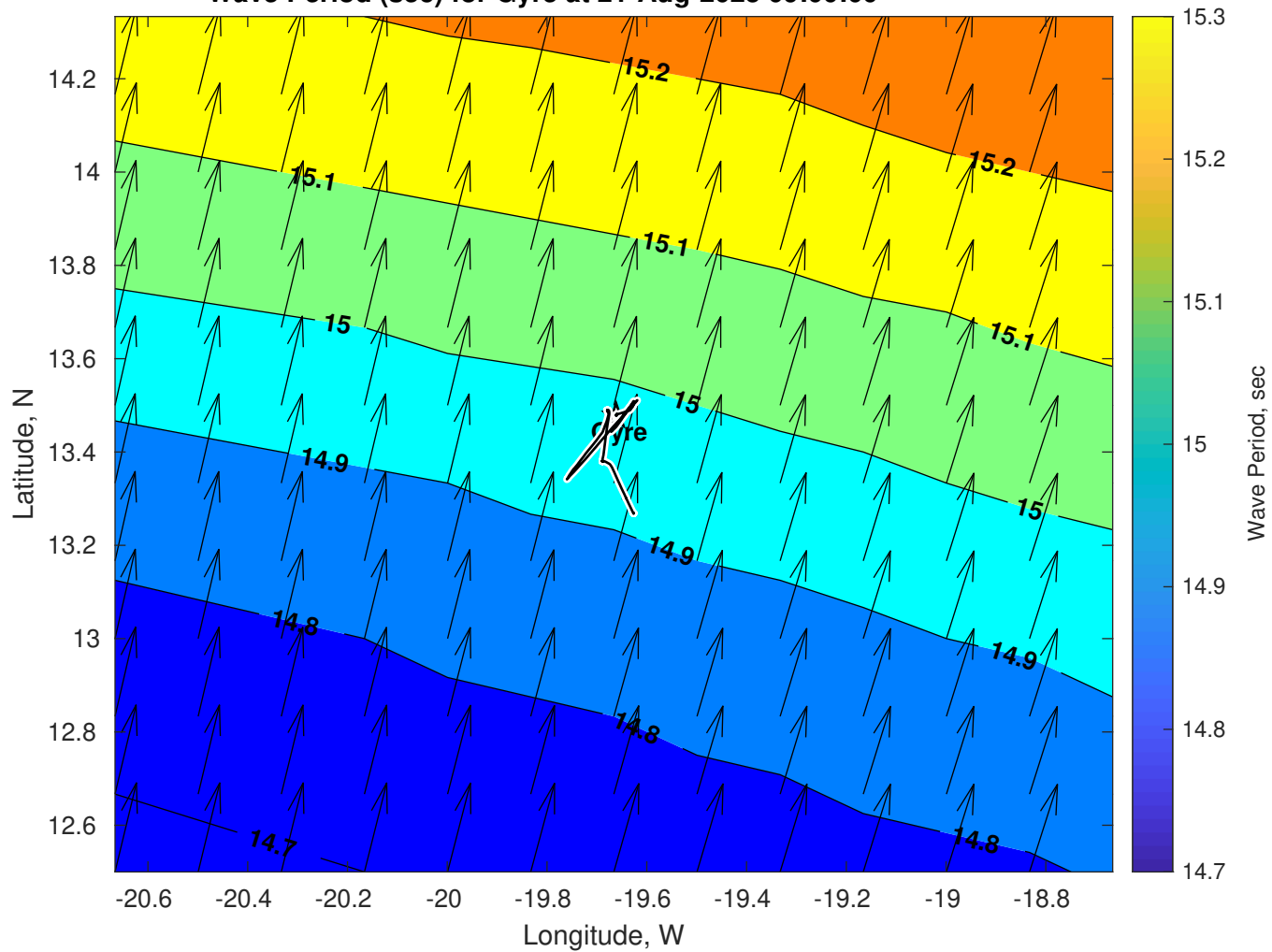
Wave Period (sec) for Gyre at 21-Aug-2025 09:00:00
