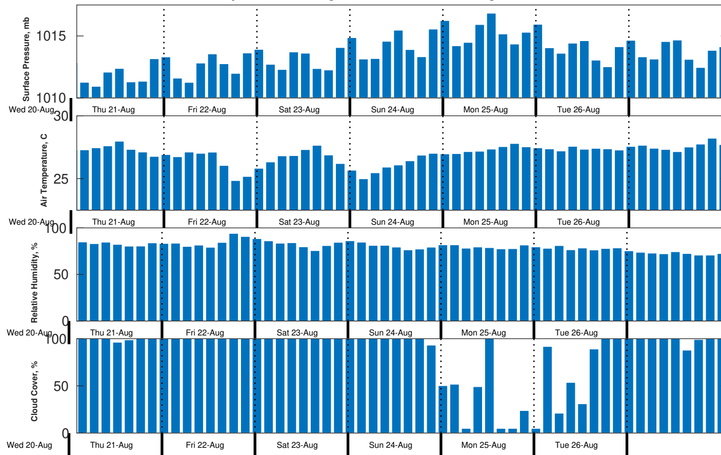
Met Forecast for Gyre from 20-Aug-2025 23:00:00 to 27-Aug-2025 23:00:00
