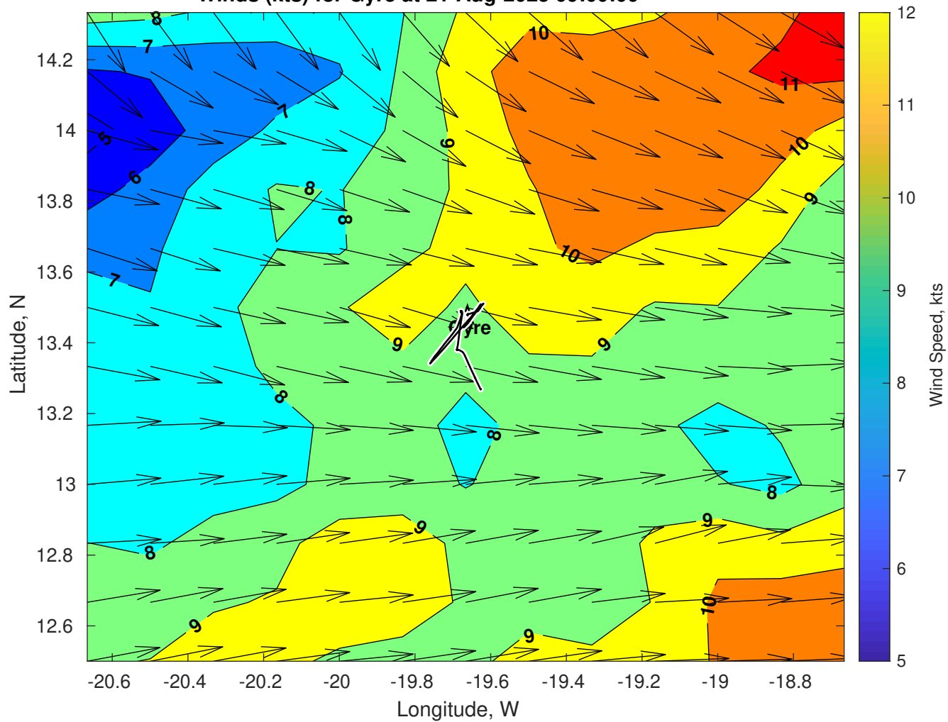
Winds (kts) for Gyre at 21-Aug-2025 09:00:00
