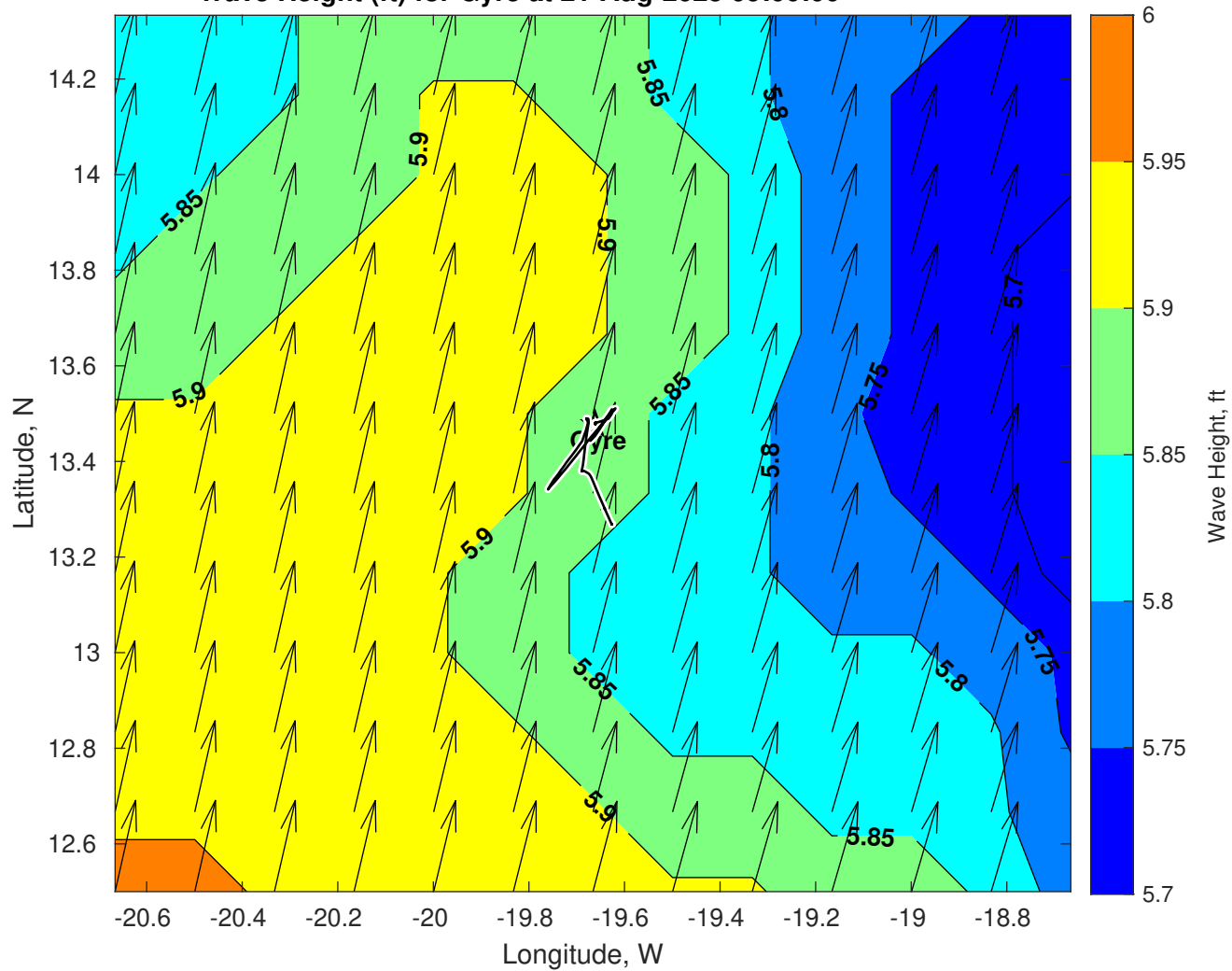
Wave Height (ft) for Gyre at 21-Aug-2025 09:00:00
