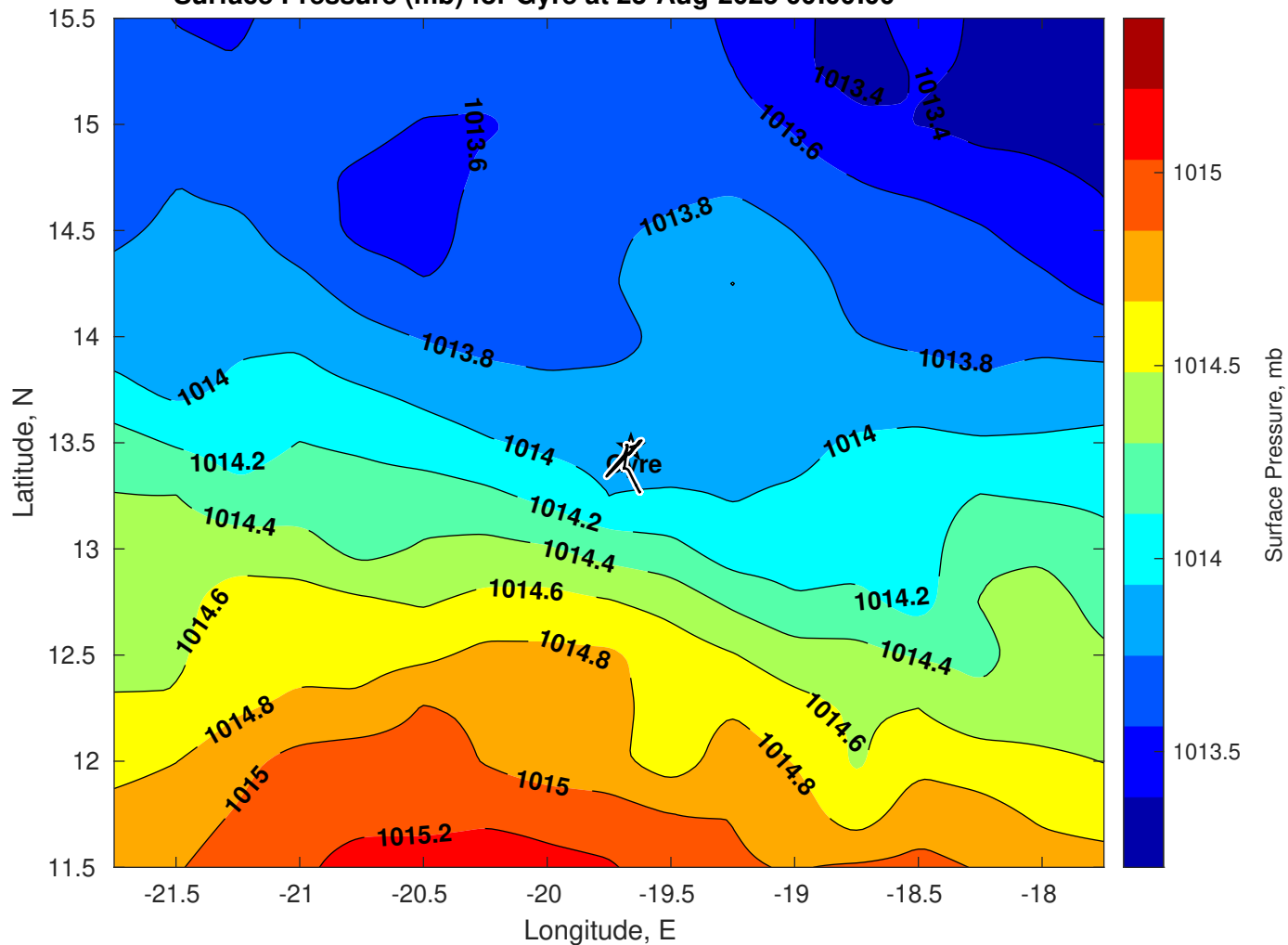
Surface Pressure (mb) for Gyre at 23-Aug-2025 00:00:00
