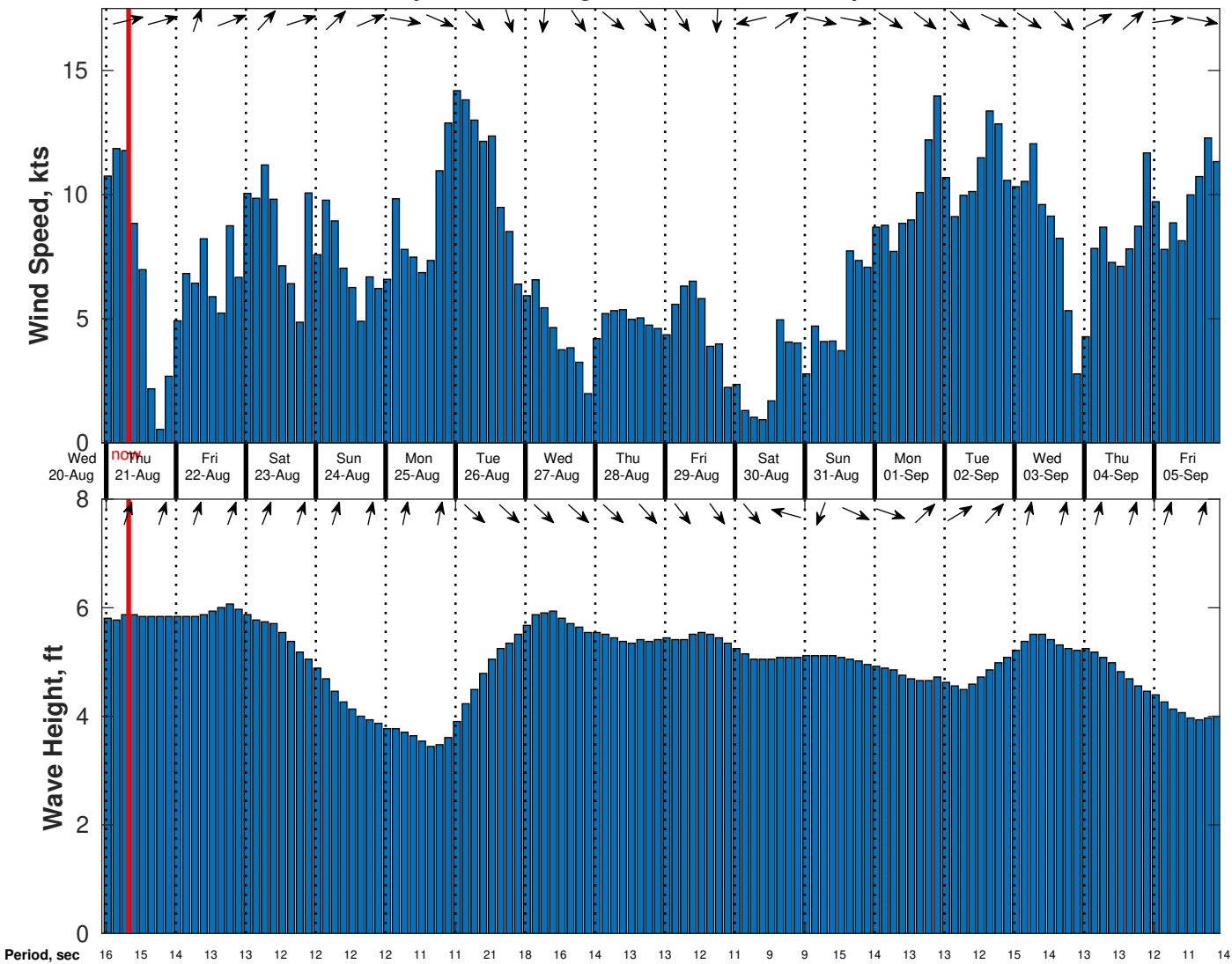
Wind & Wave Forecast for Gyre from 20-Aug-2025 23:00:00 to 05-Sep-2025 23:00:00
