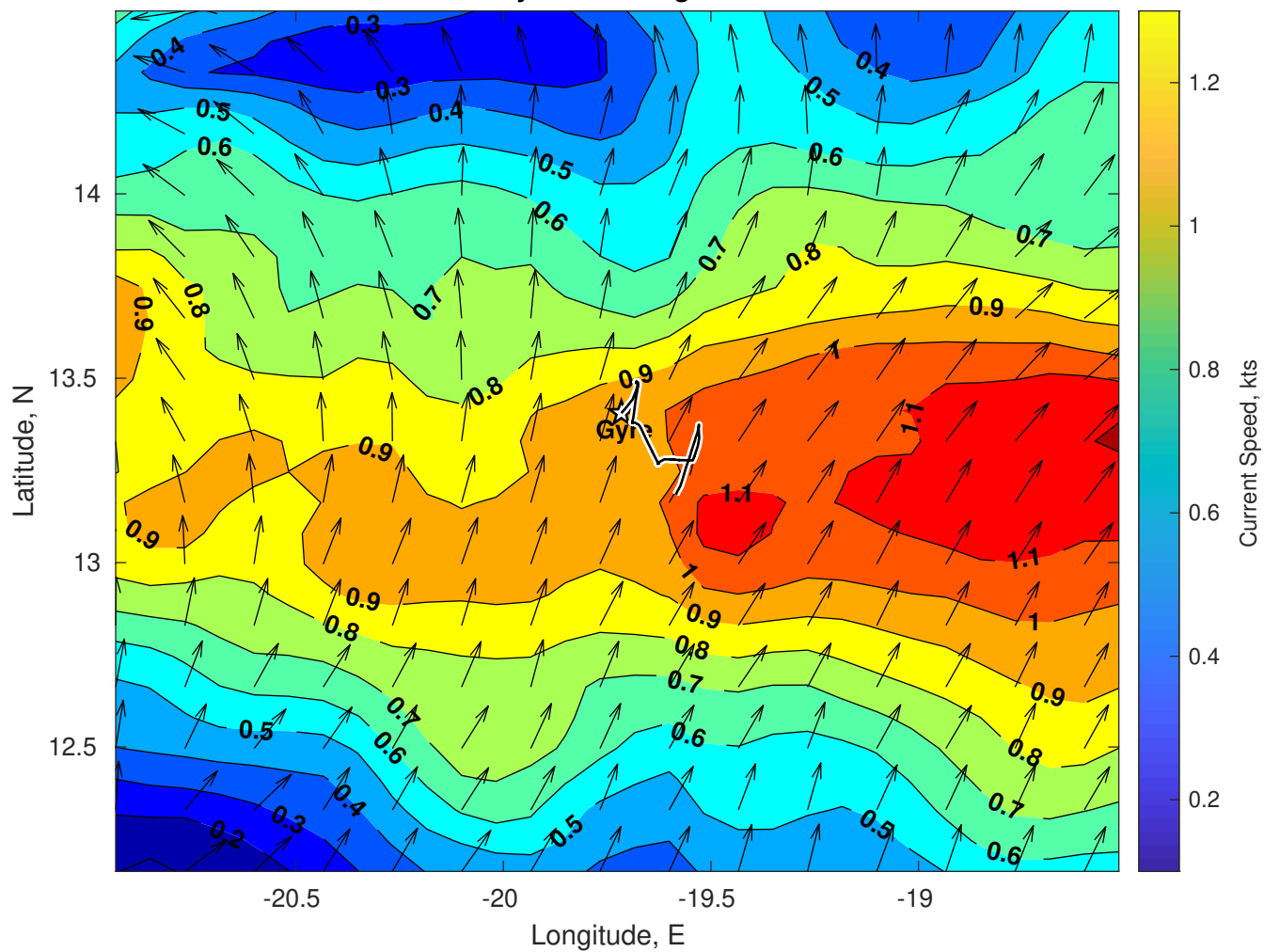
Surface Currents for Gyre at 20-Aug-2025 00:00:00
