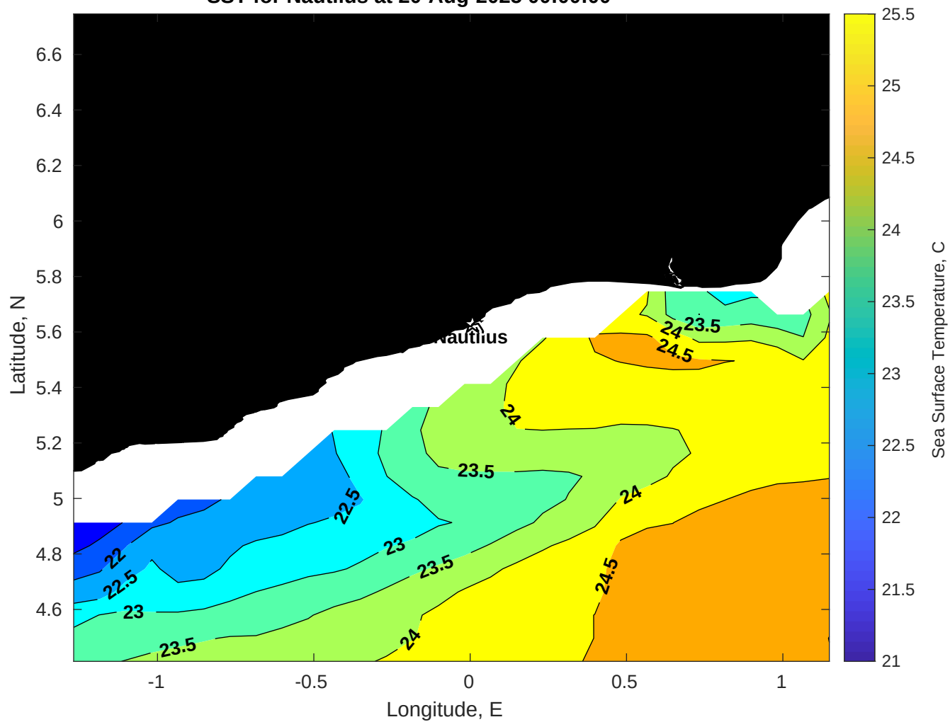
SST for Nautilus at 20-Aug-2025 00:00:00
