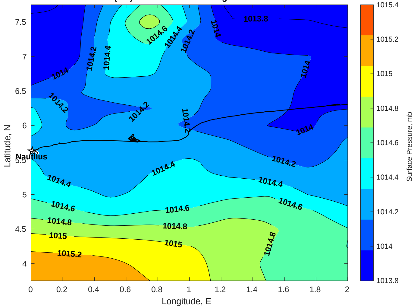
Surface Pressure (mb) for Nautilus at 23-Aug-2025 00:00:00
