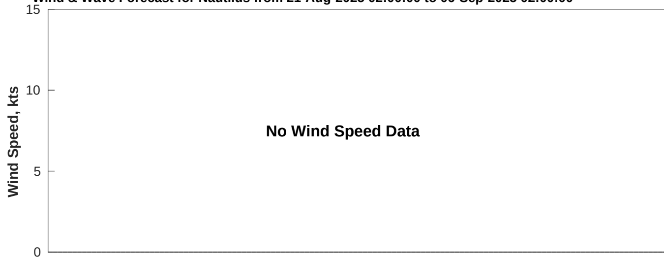
Wind & Wave Forecast for Nautilus from 21-Aug-2025 02:00:00 to 06-Sep-2025 02:00:00
