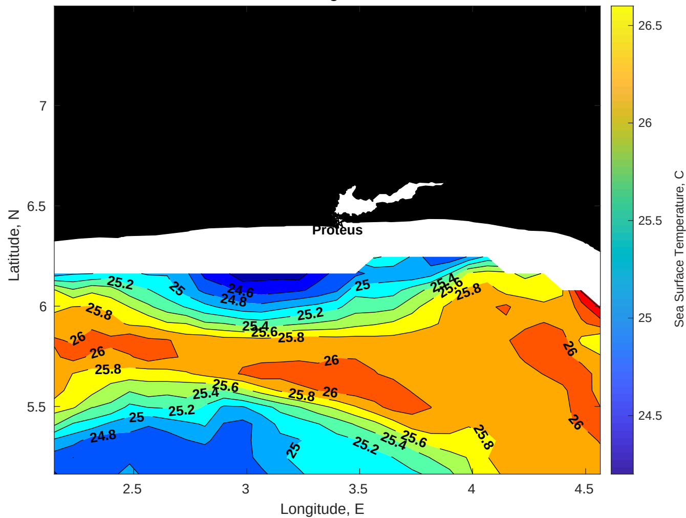
SST for Proteus at 20-Aug-2025 00:00:00
