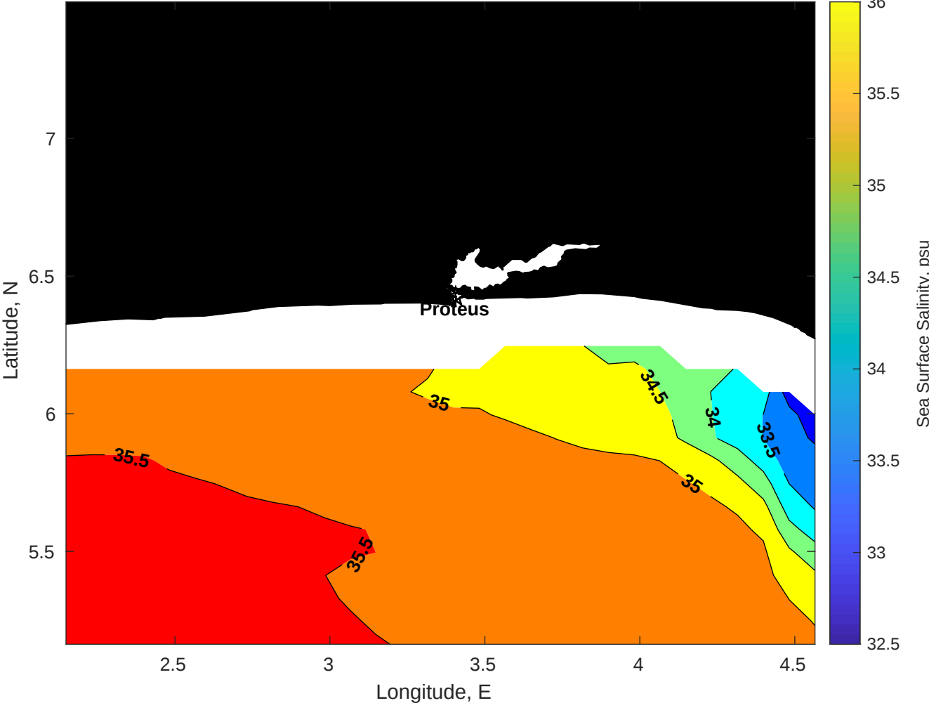
Surface Salinity for Proteus at 20-Aug-2025 00:00:00
