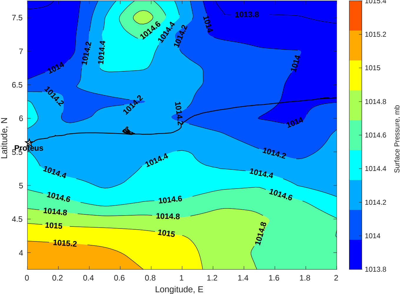
Surface Pressure (mb) for Proteus at 23-Aug-2025 00:00:00
