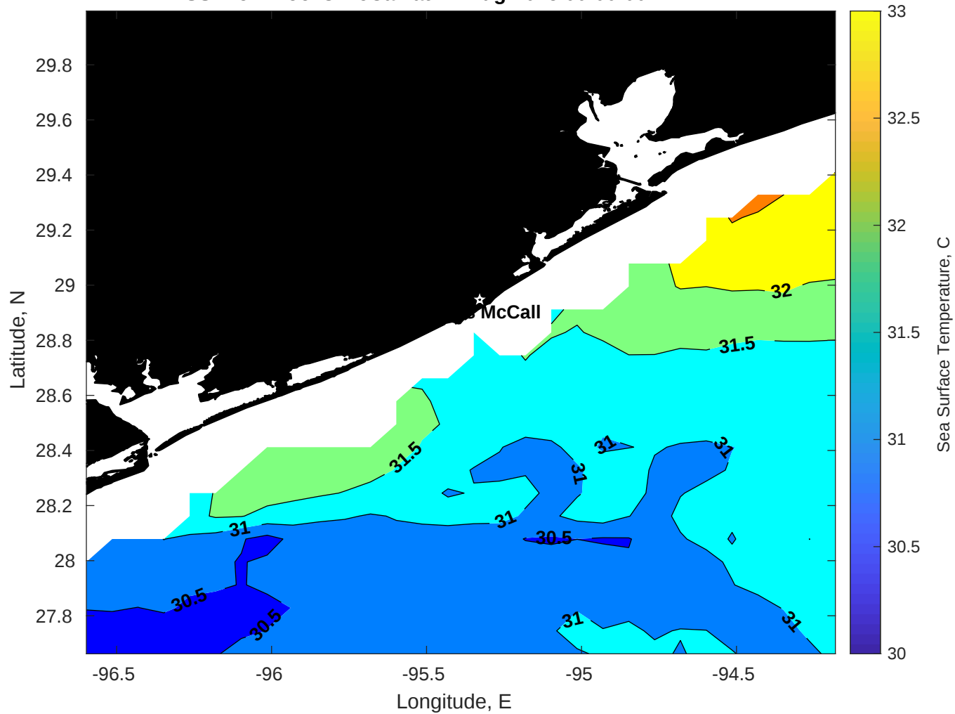
SST for Brooks McCall at 21-Aug-2025 00:00:00
