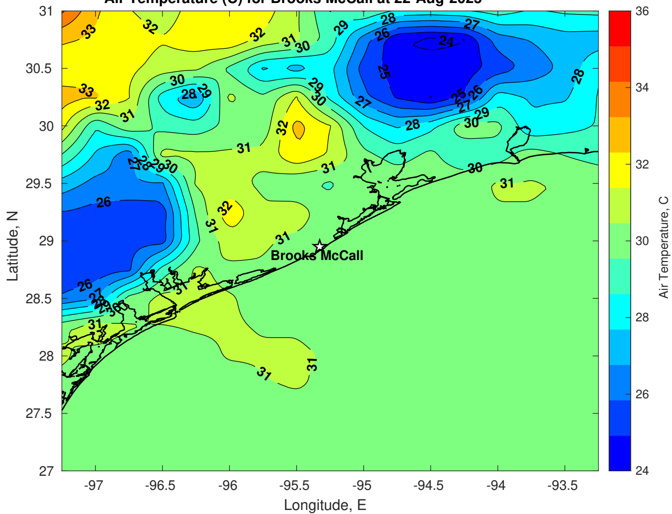
Air Temperature (C) for Brooks McCall at 22-Aug-2025
