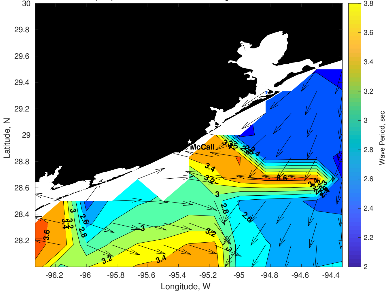
Wave Period (sec) for Brooks McCall at 22-Aug-2025 09:00:00
