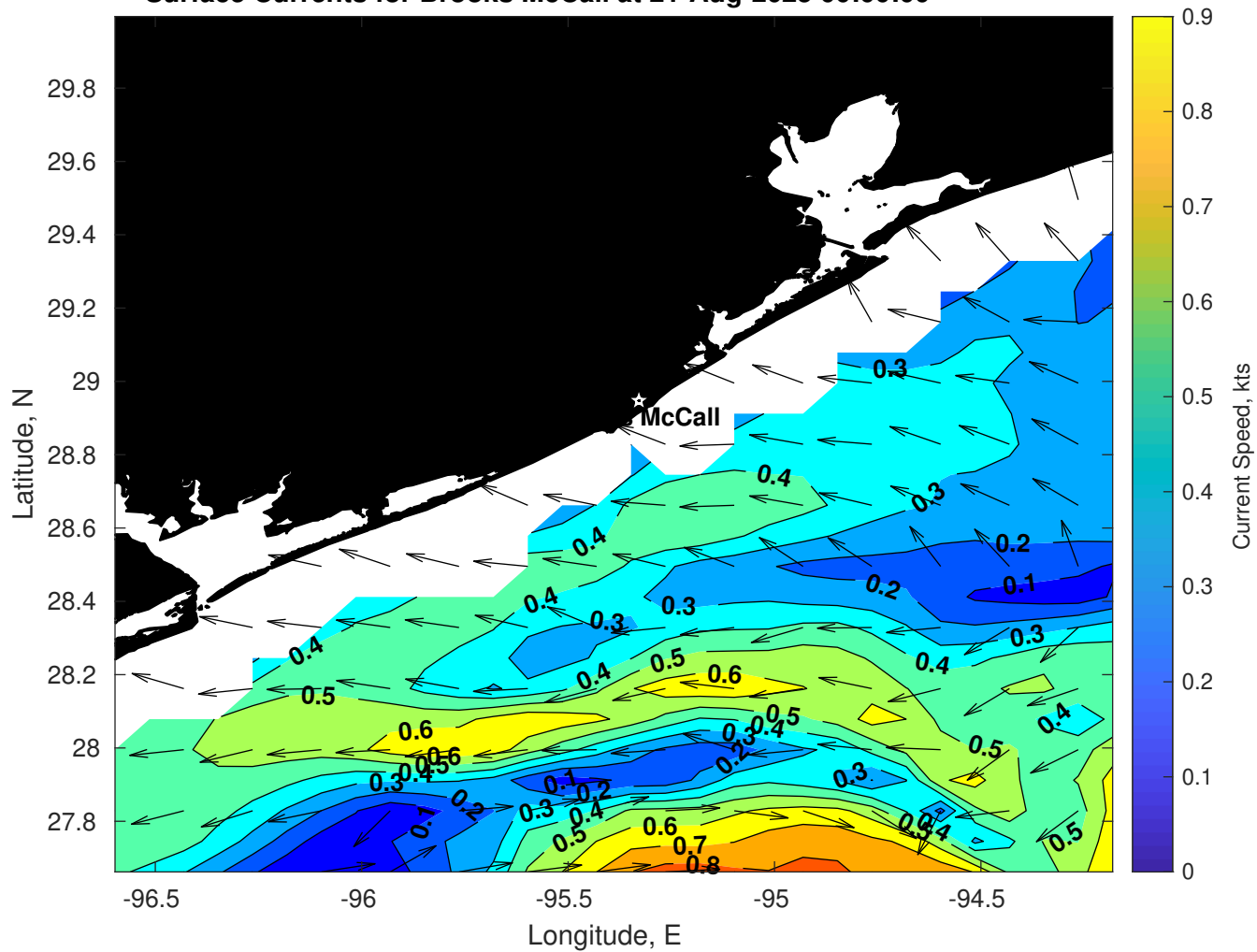
Surface Currents for Brooks McCall at 21-Aug-2025 00:00:00
