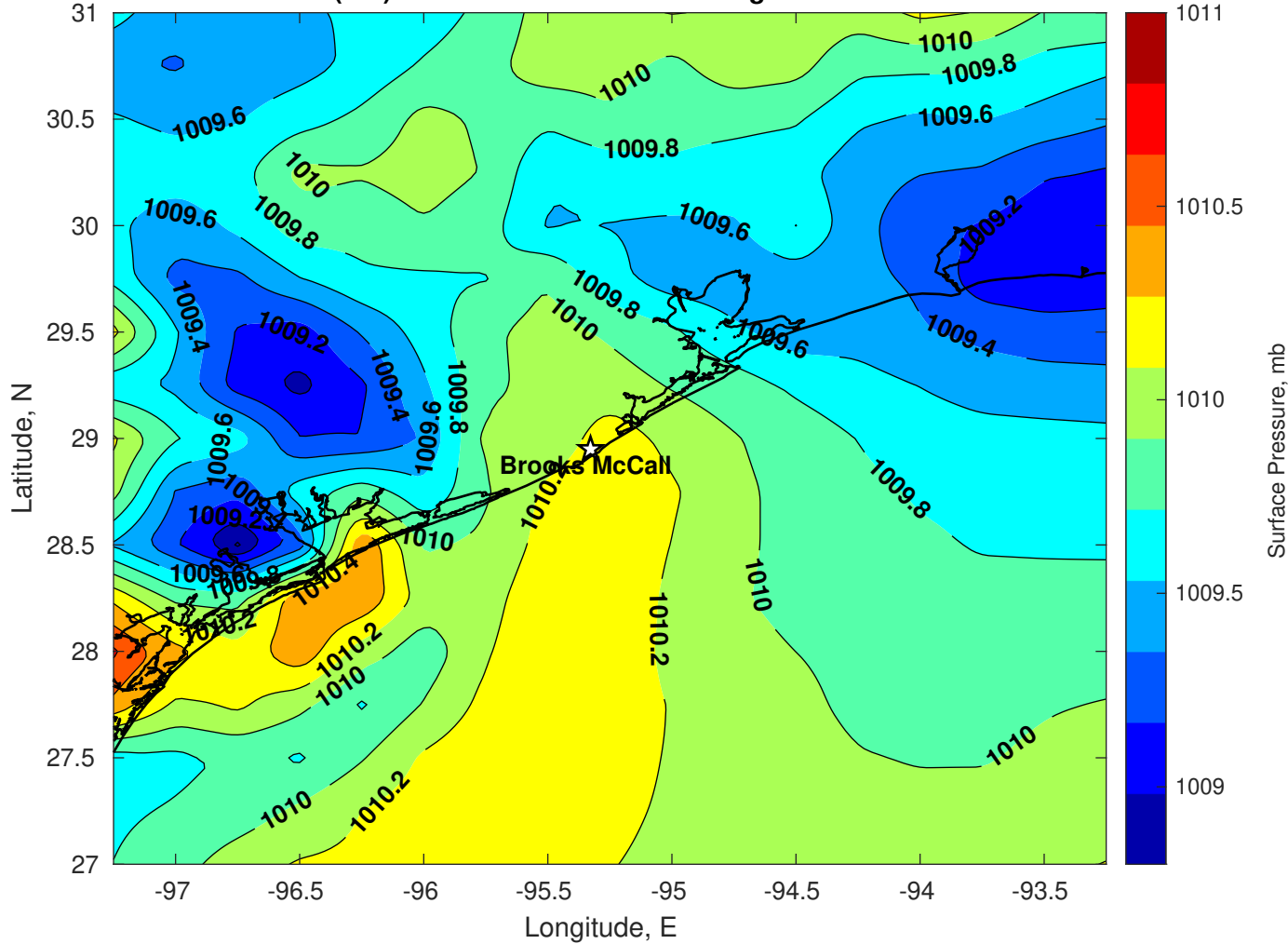
Surface Pressure (mb) for Brooks McCall at 22-Aug-2025 00:00:00
