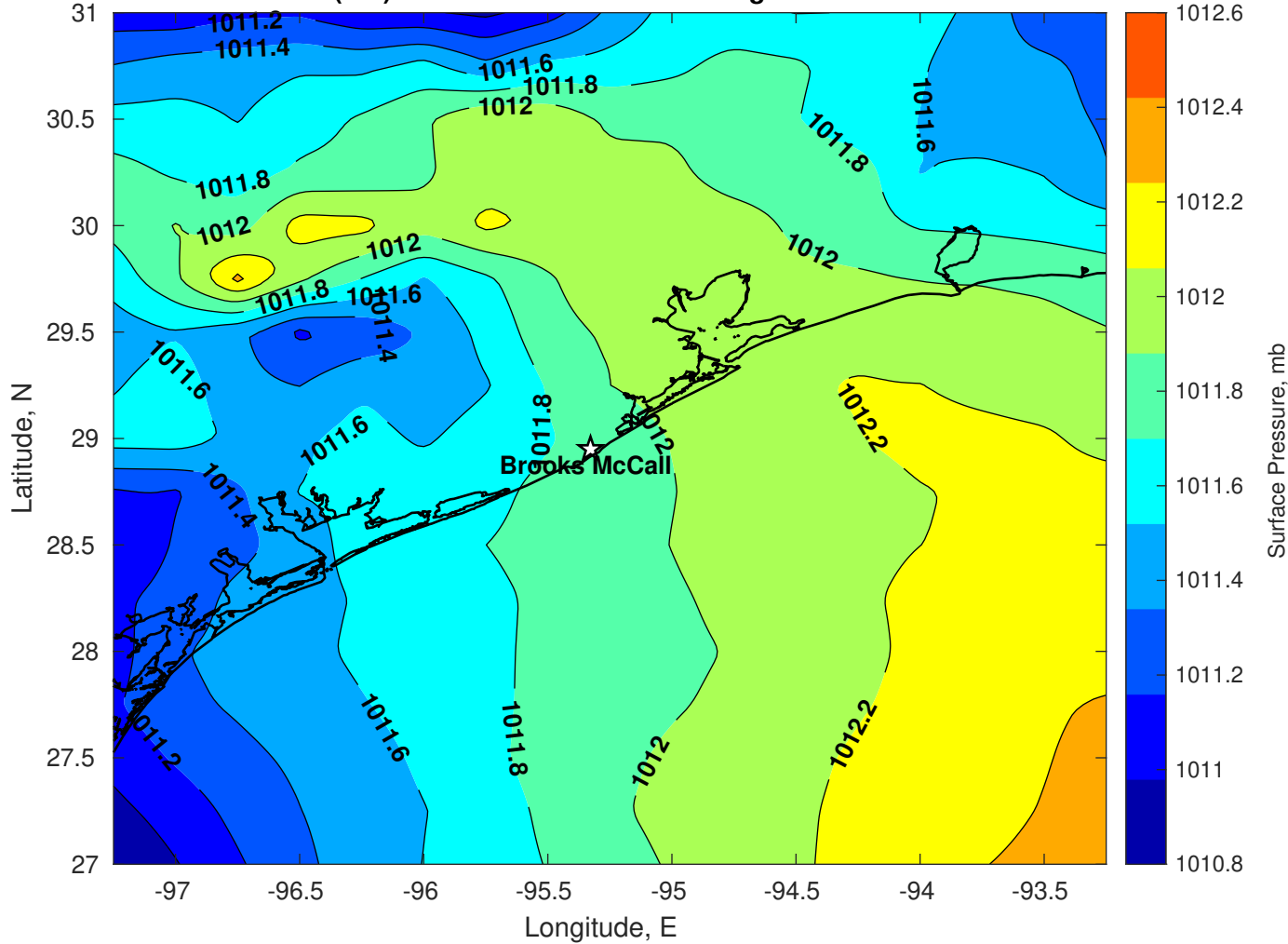
Surface Pressure (mb) for Brooks McCall at 24-Aug-2025 00:00:00
