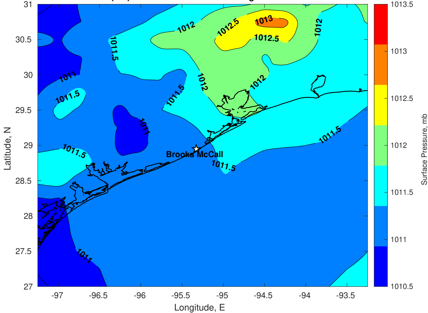
Surface Pressure (mb) for Brooks McCall at 23-Aug-2025 00:00:00
