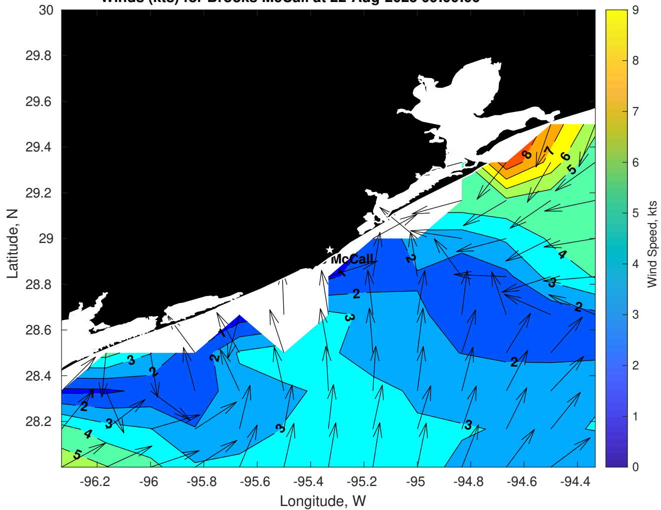
Winds (kts) for Brooks McCall at 22-Aug-2025 09:00:00
