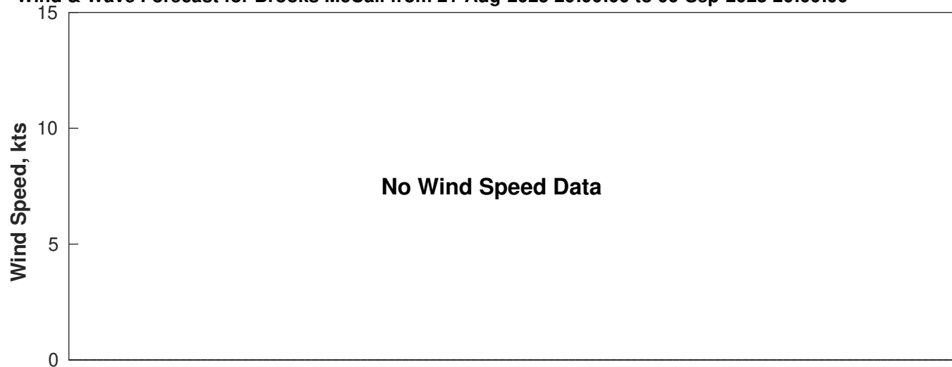
Wind & Wave Forecast for Brooks McCall from 21-Aug-2025 20:00:00 to 06-Sep-2025 20:00:00
