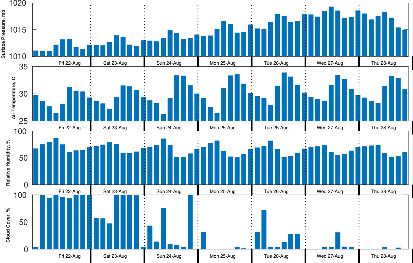
Met Forecast for Brooks McCall from 22-Aug-2025 00:00:00 to 29-Aug-2025 00:00:00
