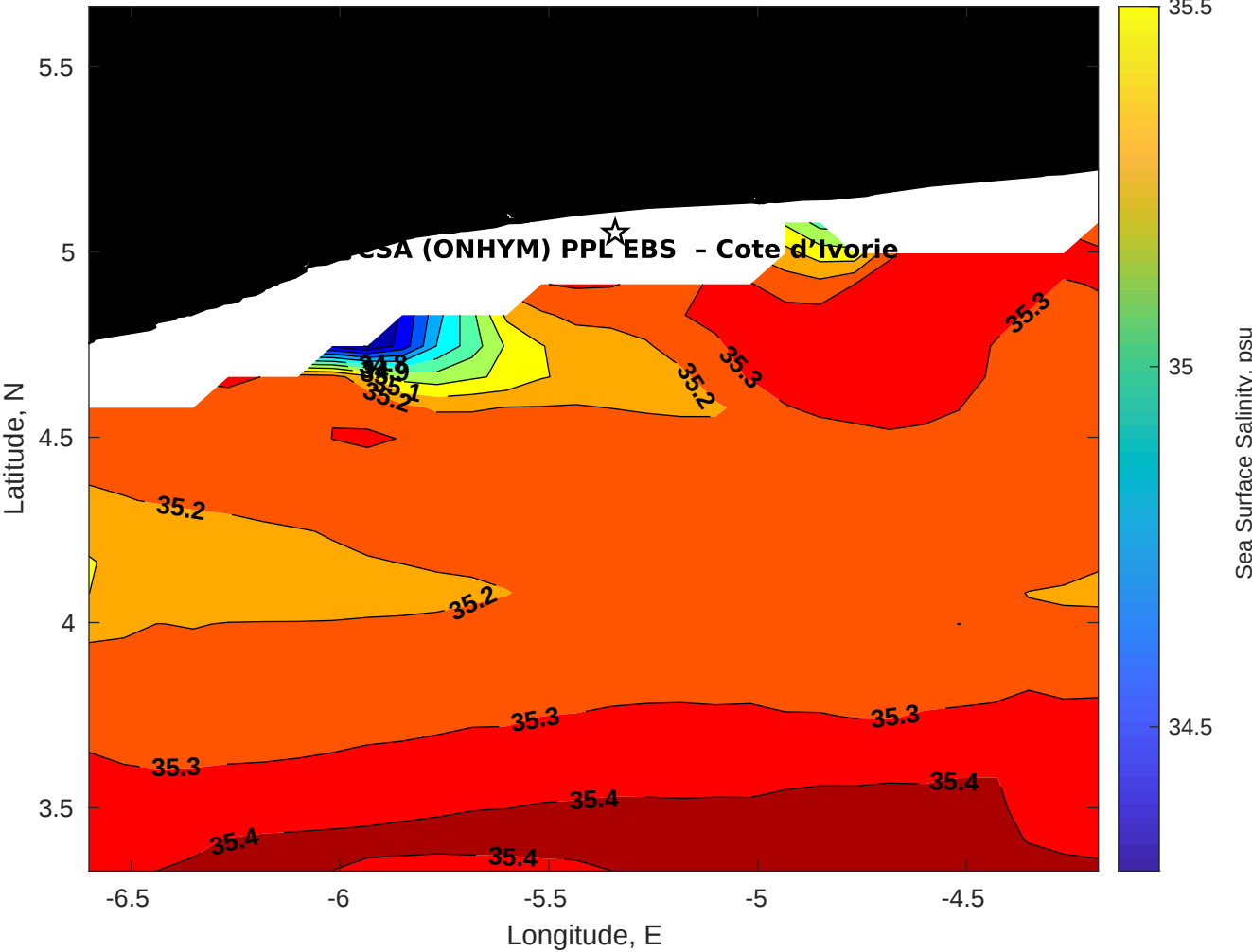
Surface Salinity for CSA (ONHYM) PPL EBS - Cote d'Ivoire at 21-Aug-2025 00:00:00
