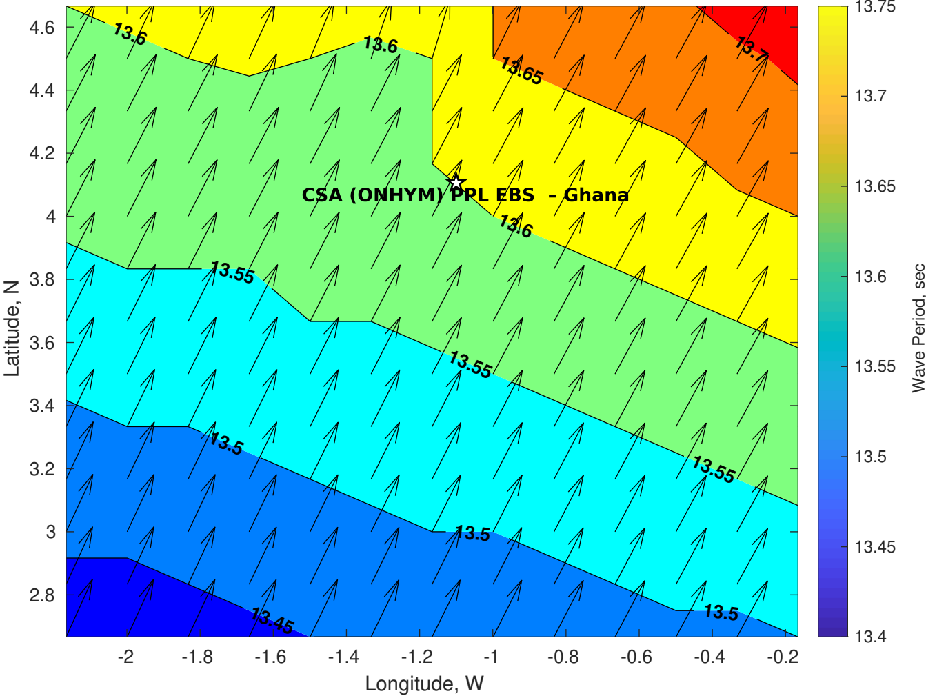
Wave Period (sec) for CSA (ONHYM) PPL EBS - Ghana at 22-Aug-2025 09:00:00
