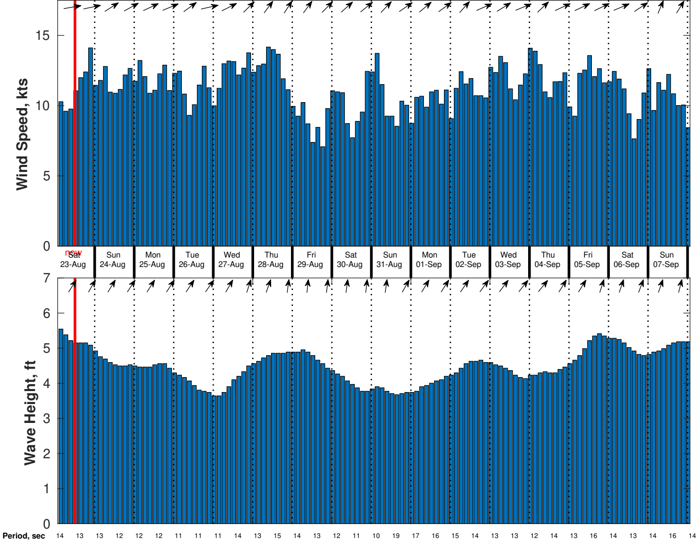
Wind & Wave Forecast for CSA (ONHYM) PPL EBS - Ghana from 22-Aug-2025 02:00:00 to 07-Sep-2025 02:00:00
