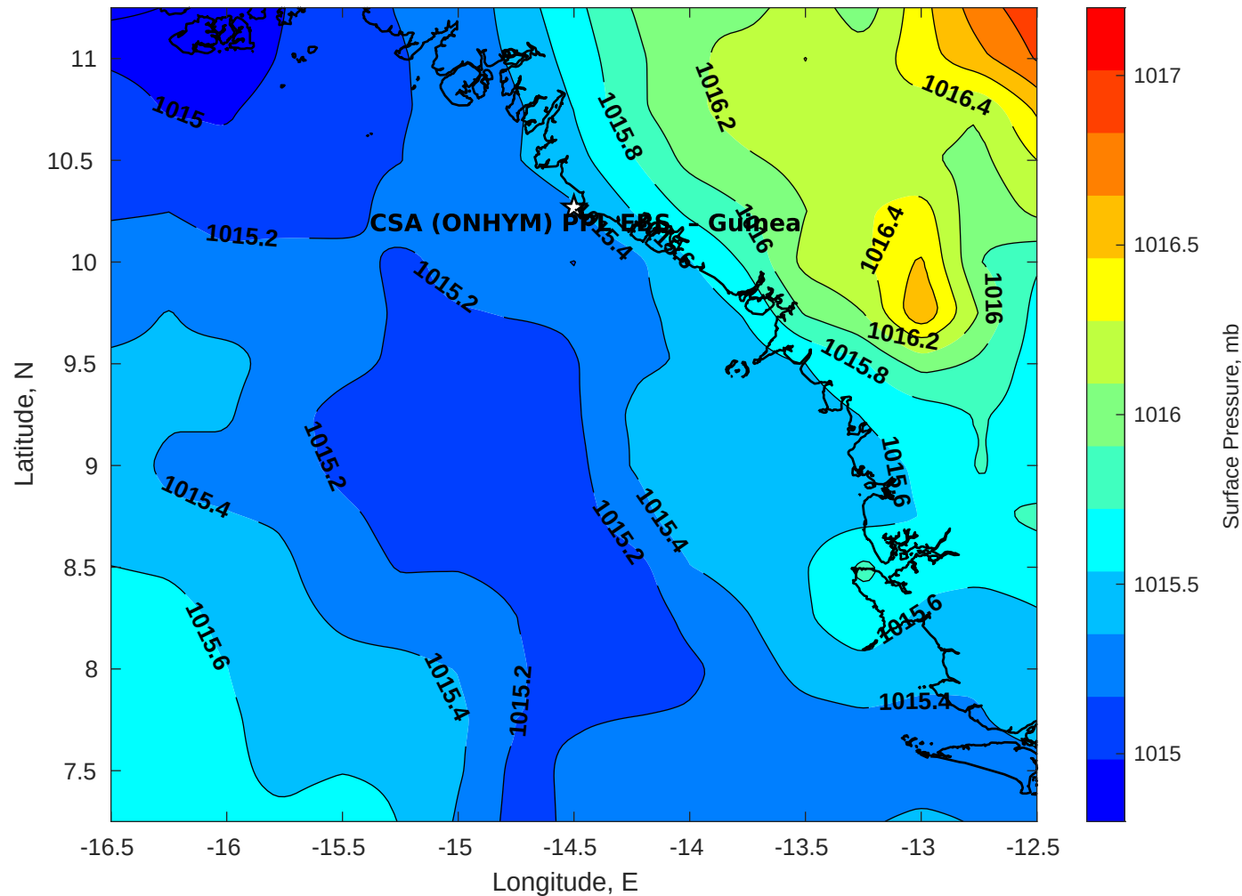
Surface Pressure (mb) for CSA (ONHYM) PPL EBS - Guinea at 23-Aug-2025 00:00:00
