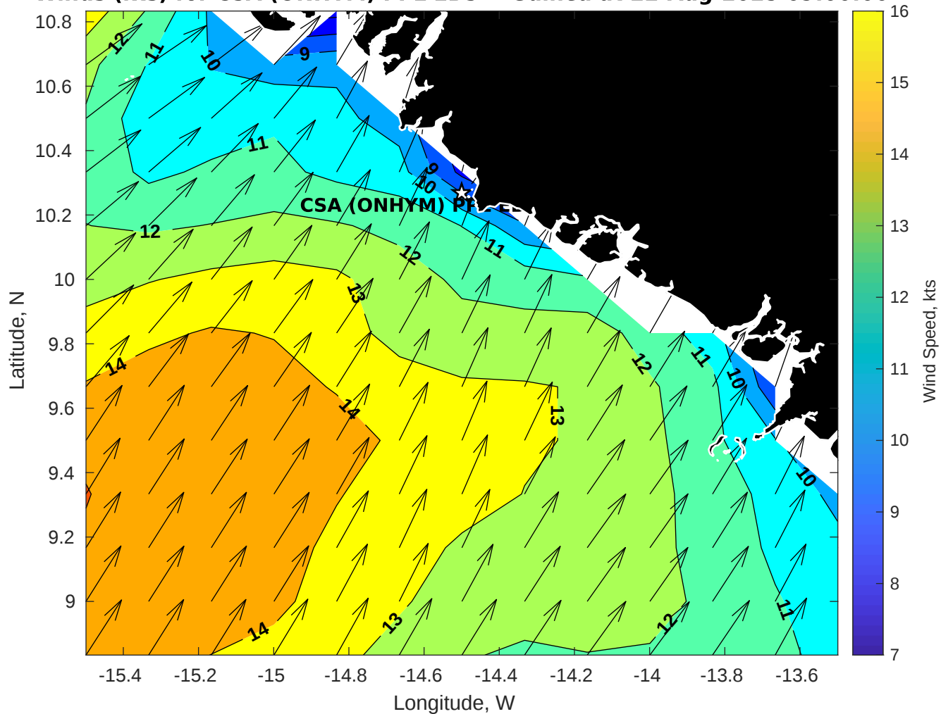
Winds (kts) for CSA (ONHYM) PPL EBS - Guinea at 22-Aug-2025 09:00:00
