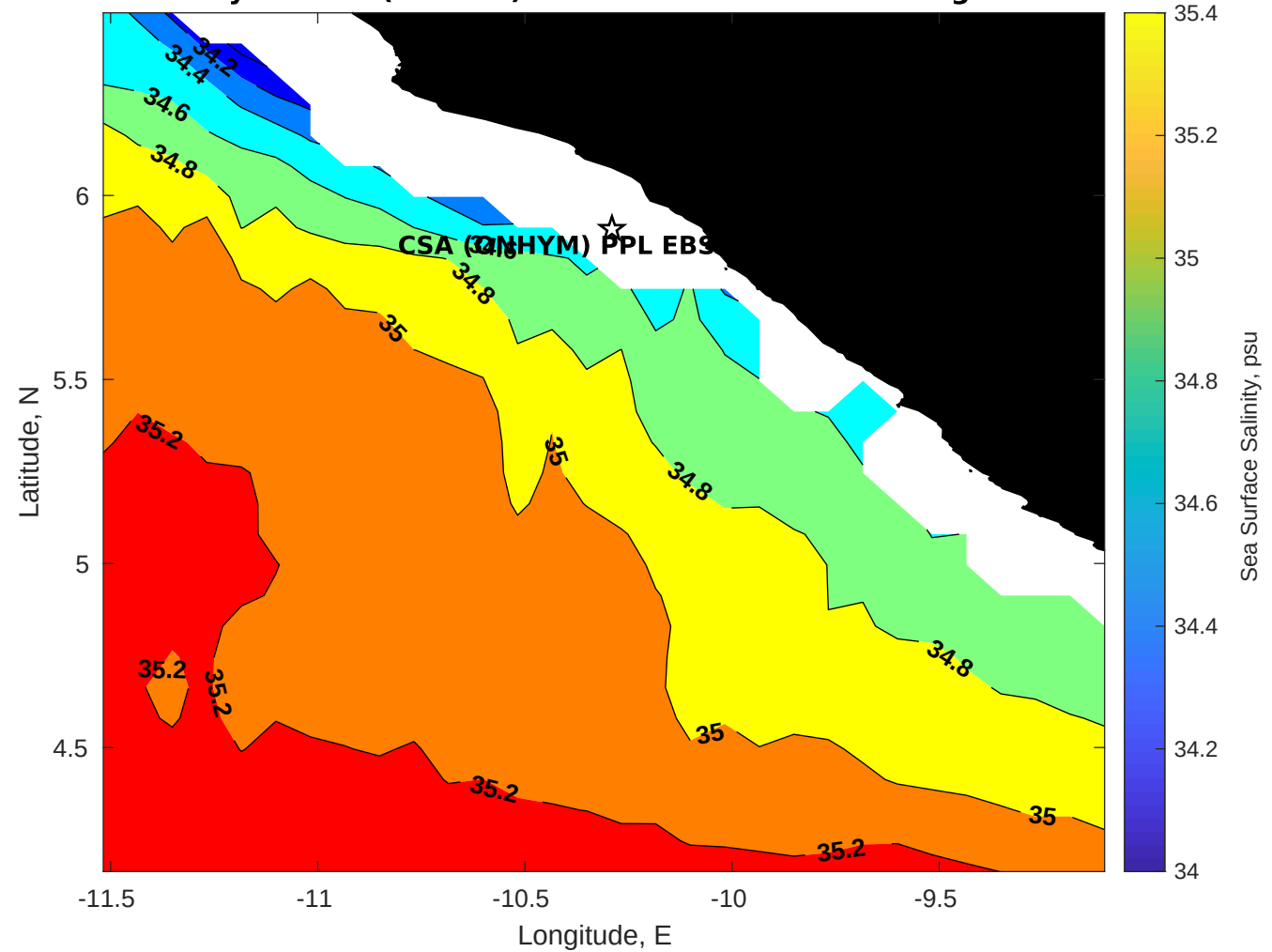
Surface Salinity for CSA (ONHYM) PPL EBS - Liberia at 21-Aug-2025 00:00:00
