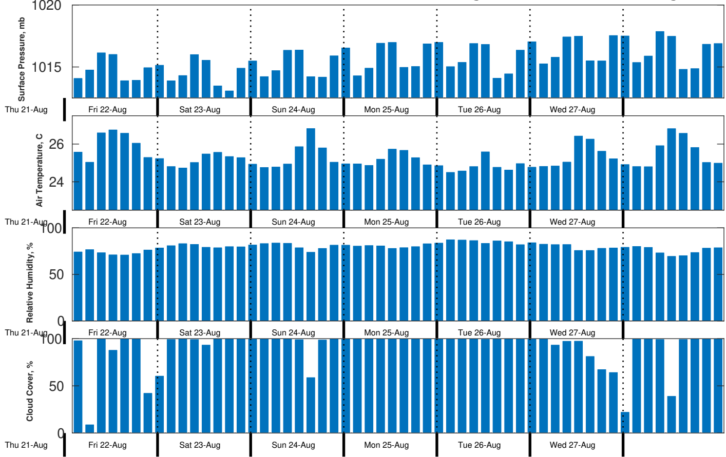
Met Forecast for CSA (ONHYM) PPL EBS - Liberia from 22-Aug-2025 00:00:00 to 29-Aug-2025 00:00:00
