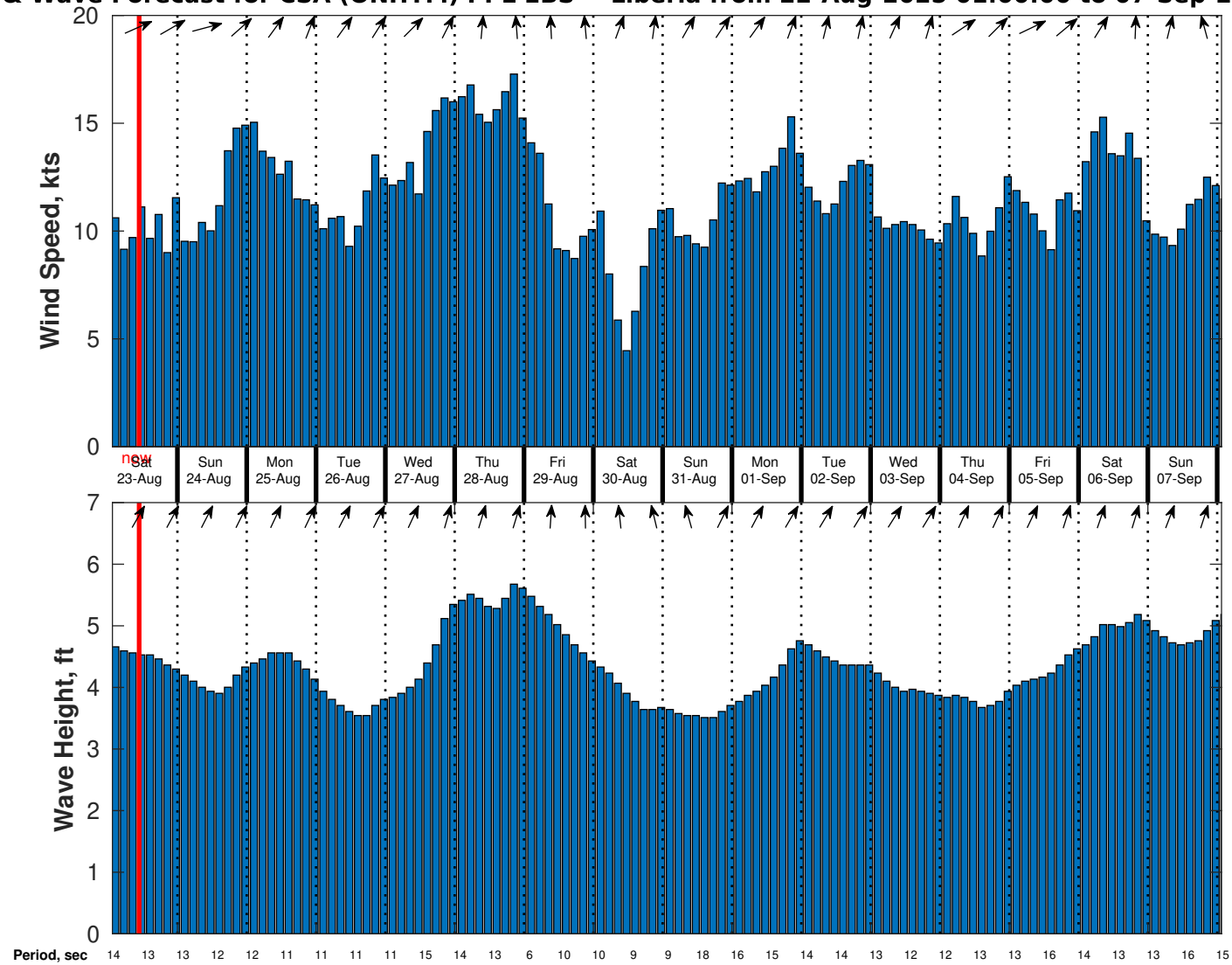
Wind & Wave Forecast for CSA (ONHYM) PPL EBS - Liberia from 22-Aug-2025 01:00:00 to 07-Sep-2025 01:00:00
