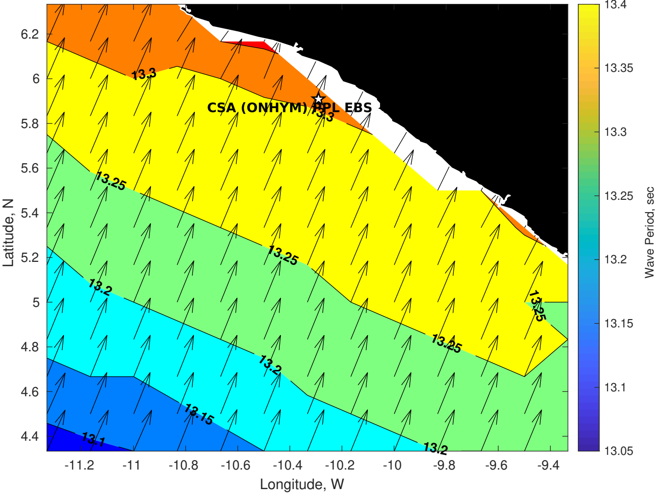
Wave Period (sec) for CSA (ONHYM) PPL EBS - Liberia at 22-Aug-2025 09:00:00
