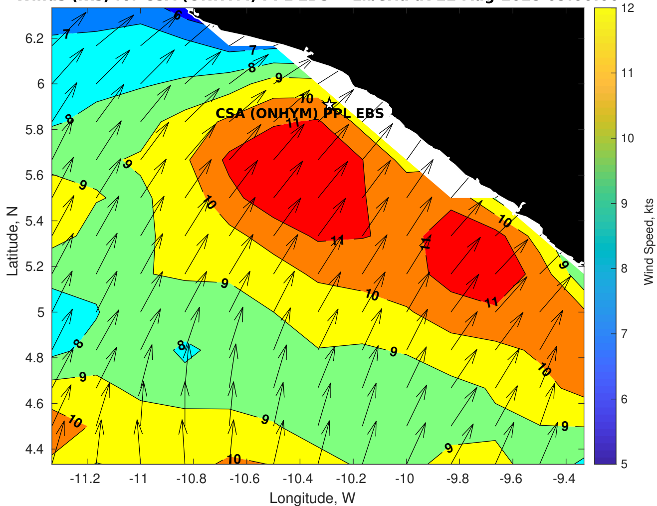
Winds (kts) for CSA (ONHYM) PPL EBS - Liberia at 22-Aug-2025 09:00:00
