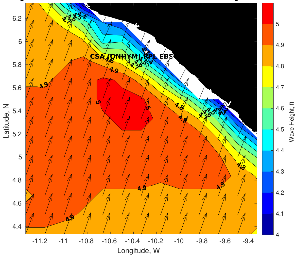
Wave Height (ft) for CSA (ONHYM) PPL EBS - Liberia at 22-Aug-2025 09:00:00
