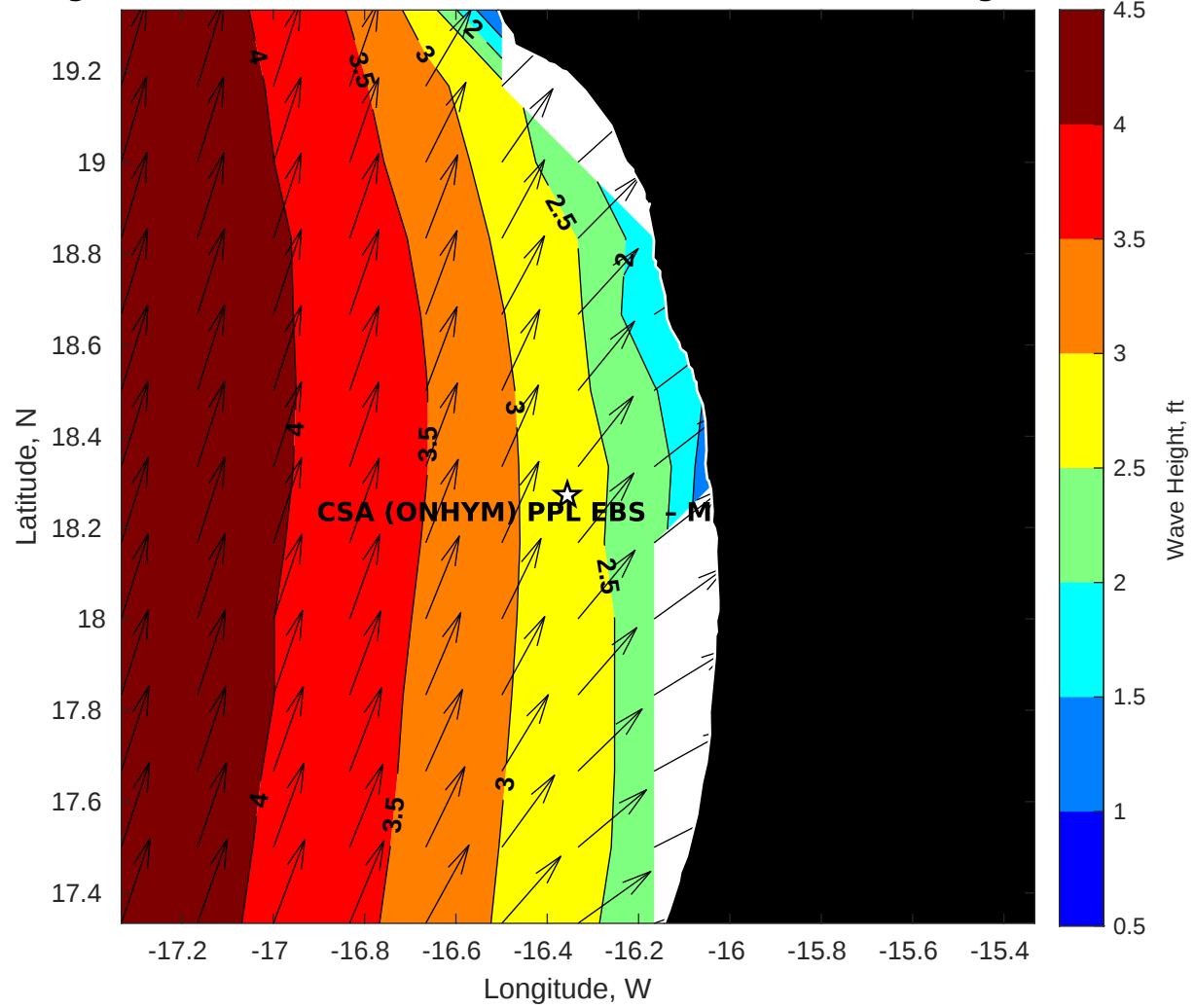
Wave Height (ft) for CSA (ONHYM) PPL EBS - Mauritania at 22-Aug-2025 09:00:00
