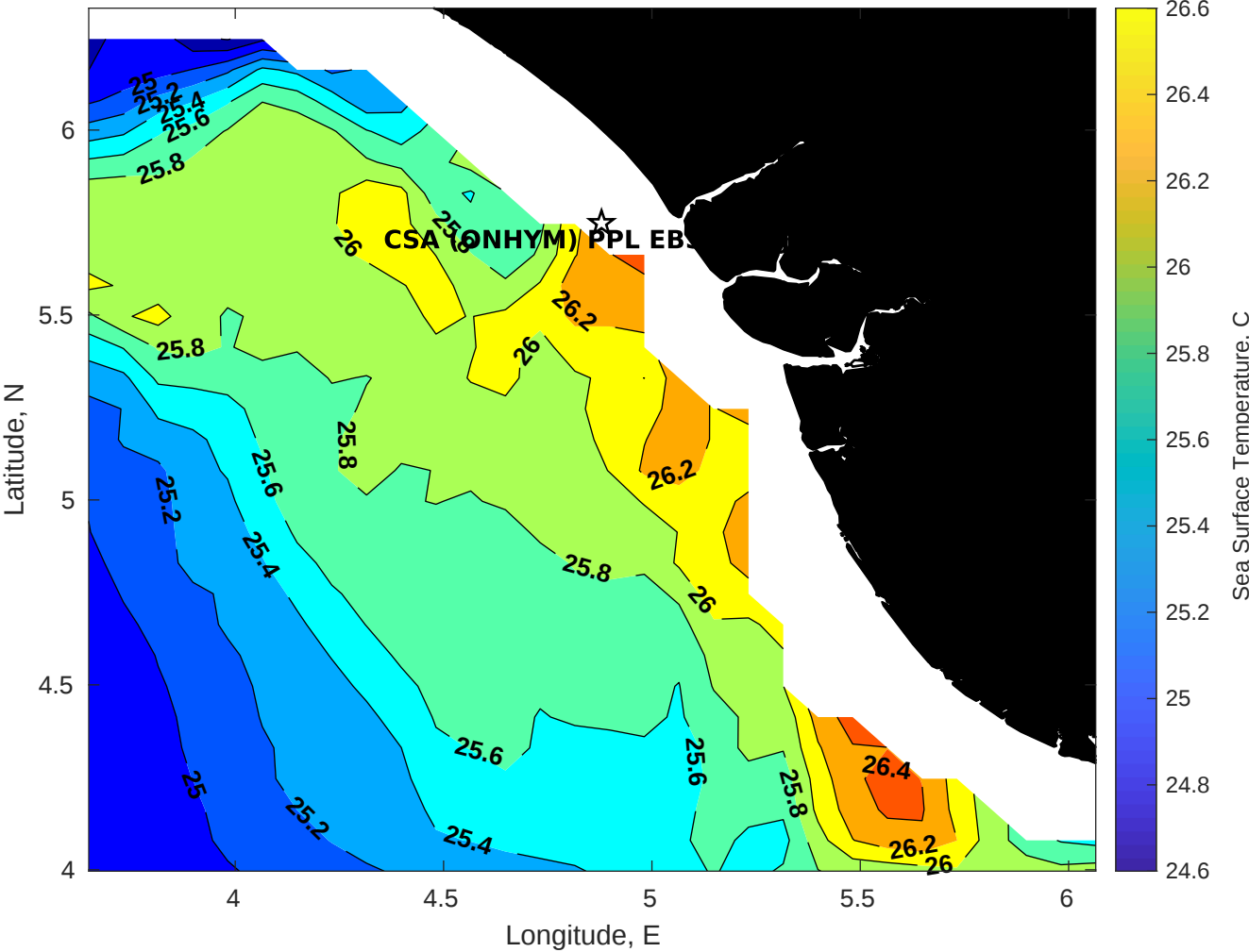
SST for CSA (ONHYM) PPL EBS - Nigeria at 21-Aug-2025 00:00:00
