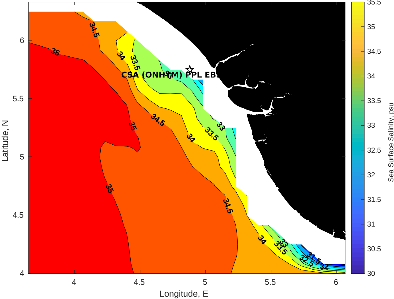
Surface Salinity for CSA (ONHYM) PPL EBS - Nigeria at 21-Aug-2025 00:00:00
