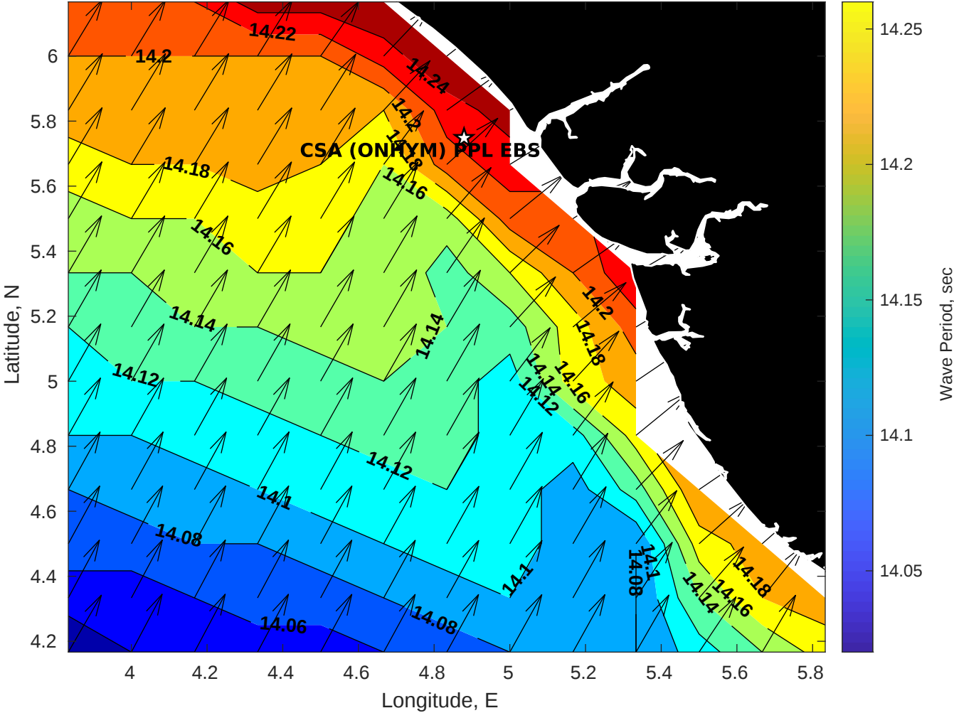
Wave Period (sec) for CSA (ONHYM) PPL EBS - Nigeria at 22-Aug-2025 09:00:00
