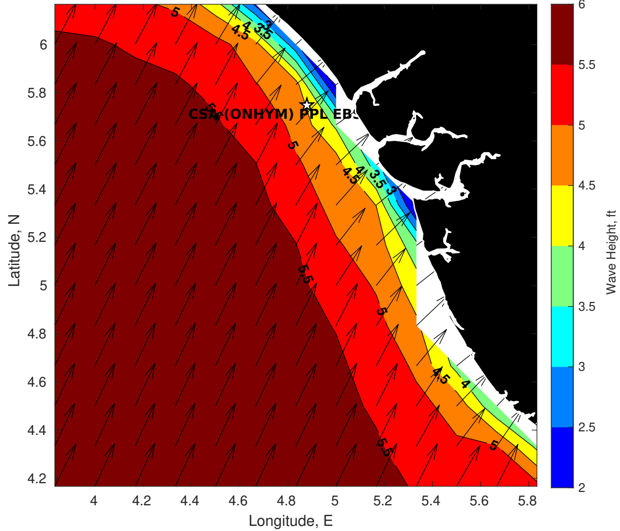
Wave Height (ft) for CSA (ONHYM) PPL EBS - Nigeria at 22-Aug-2025 09:00:00
