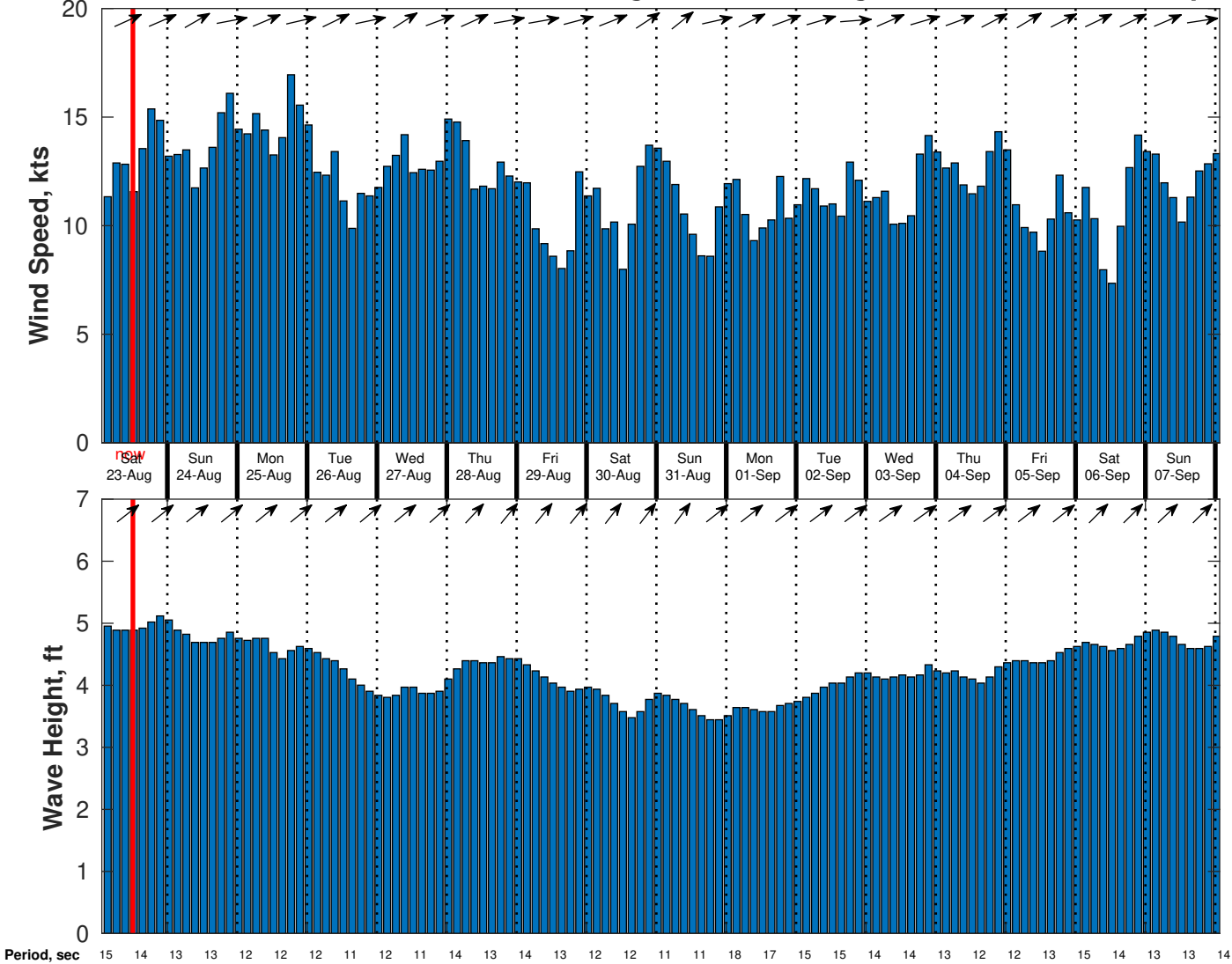
Wind & Wave Forecast for CSA (ONHYM) PPL EBS - Nigeria from 22-Aug-2025 02:00:00 to 07-Sep-2025 02:00:00
