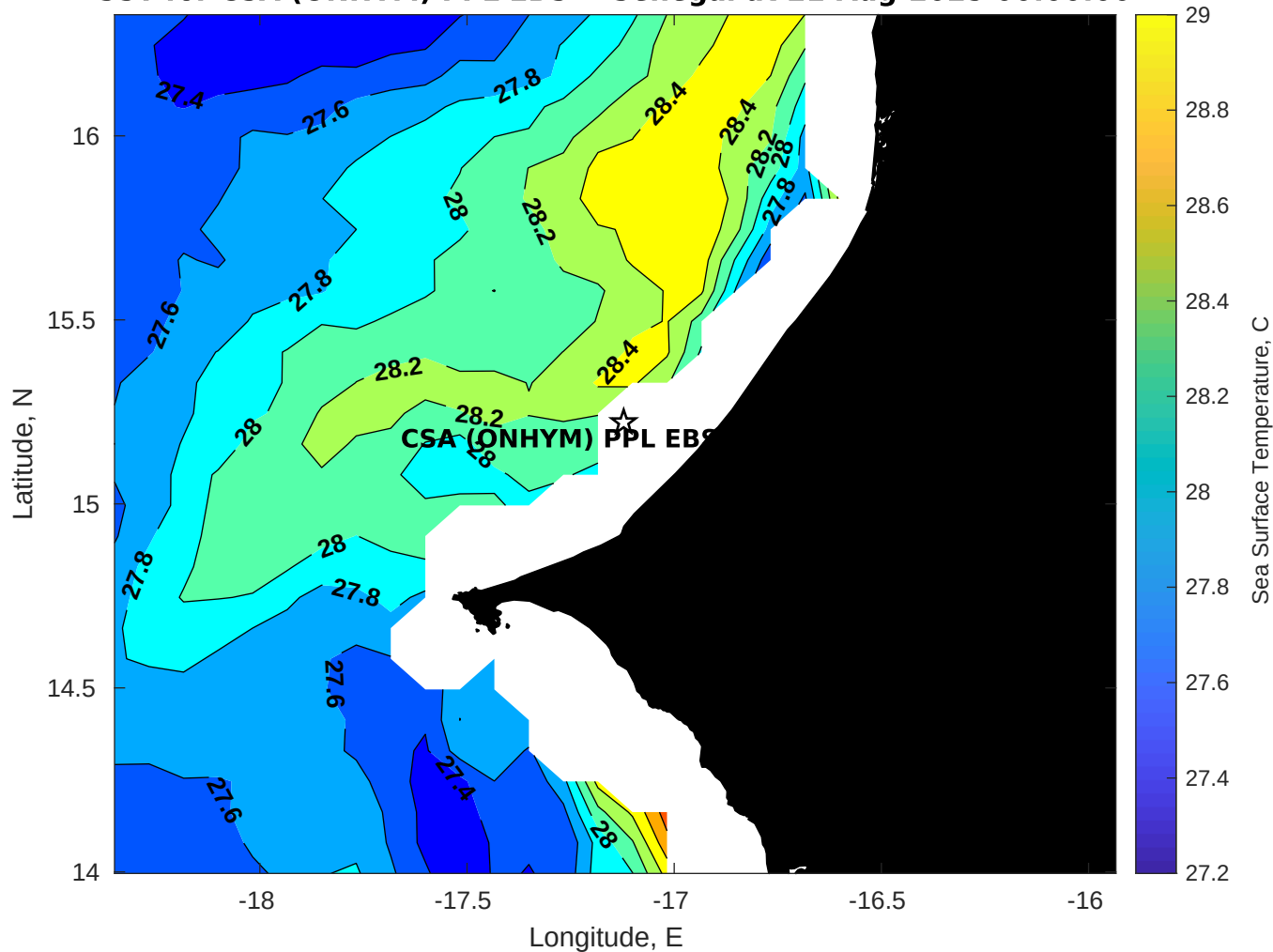
SST for CSA (ONHYM) PPL EBS - Senegal at 21-Aug-2025 00:00:00
