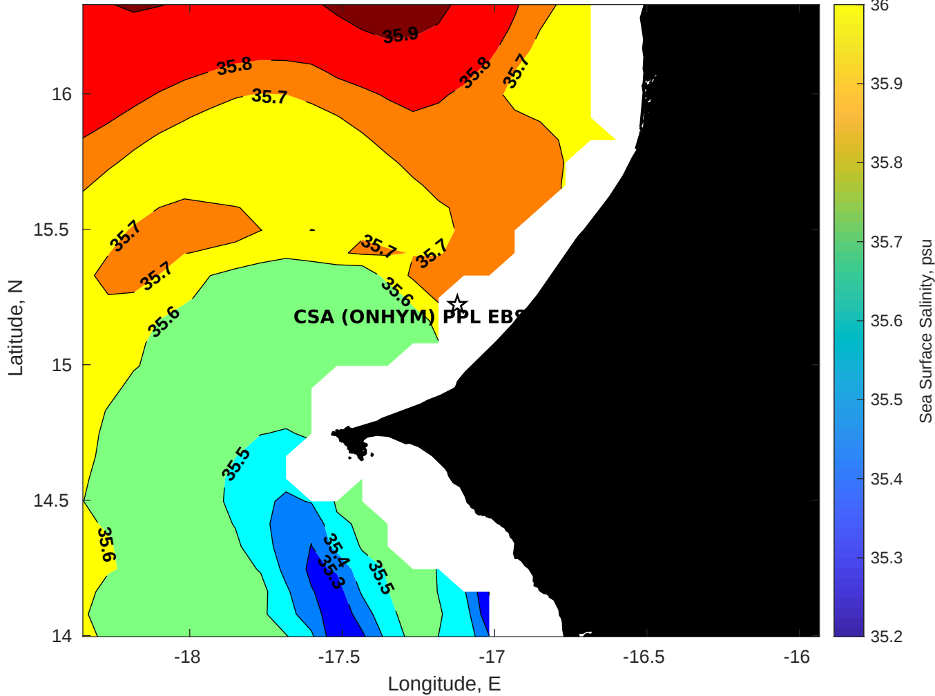
Surface Salinity for CSA (ONHYM) PPL EBS - Senegal at 21-Aug-2025 00:00:00
