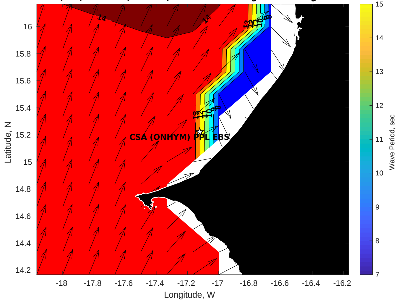
Wave Period (sec) for CSA (ONHYM) PPL EBS - Senegal at 22-Aug-2025 09:00:00
