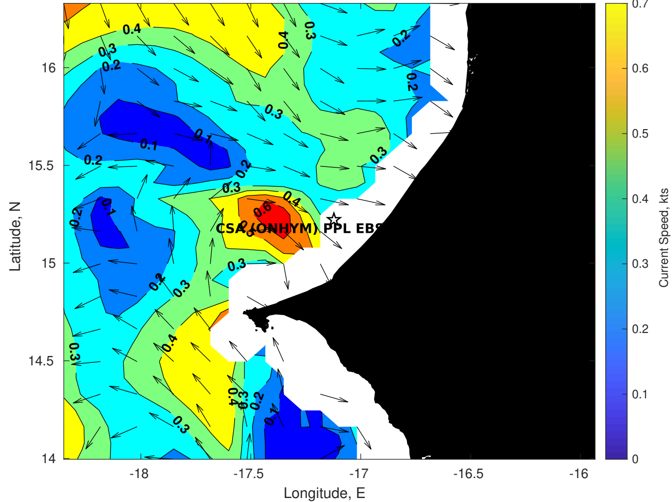
Surface Currents for CSA (ONHYM) PPL EBS - Senegal at 21-Aug-2025 00:00:00
