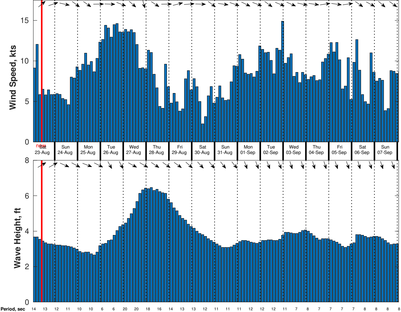
Wind & Wave Forecast for CSA (ONHYM) PPL EBS - Senegal from 22-Aug-2025 01:00:00 to 07-Sep-2025 01:00:00
