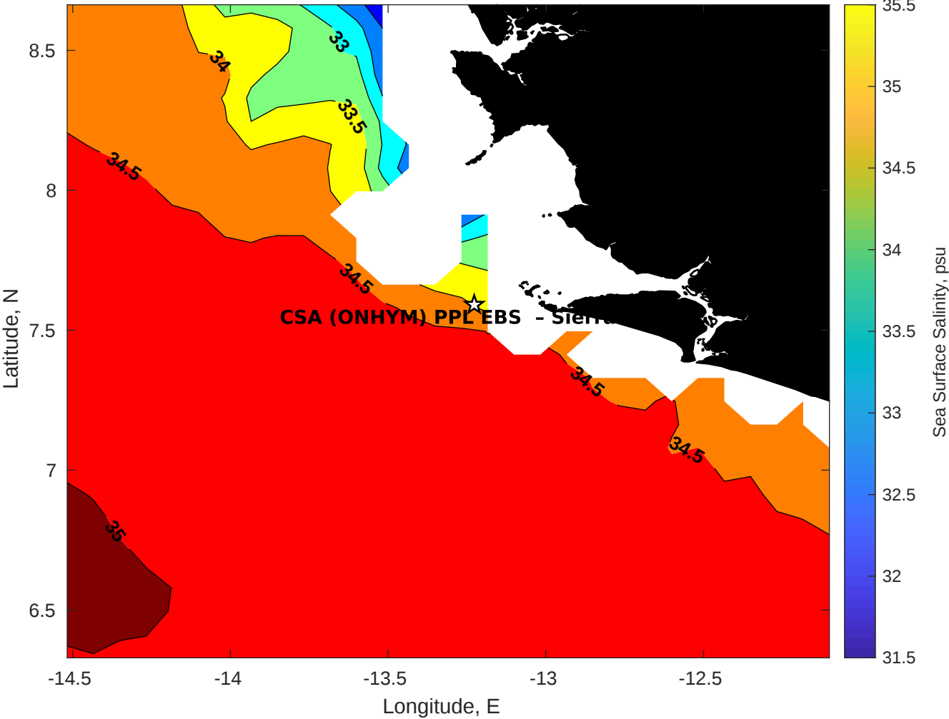
Surface Salinity for CSA (ONHYM) PPL EBS - Sierra Leone at 21-Aug-2025 00:00:00
