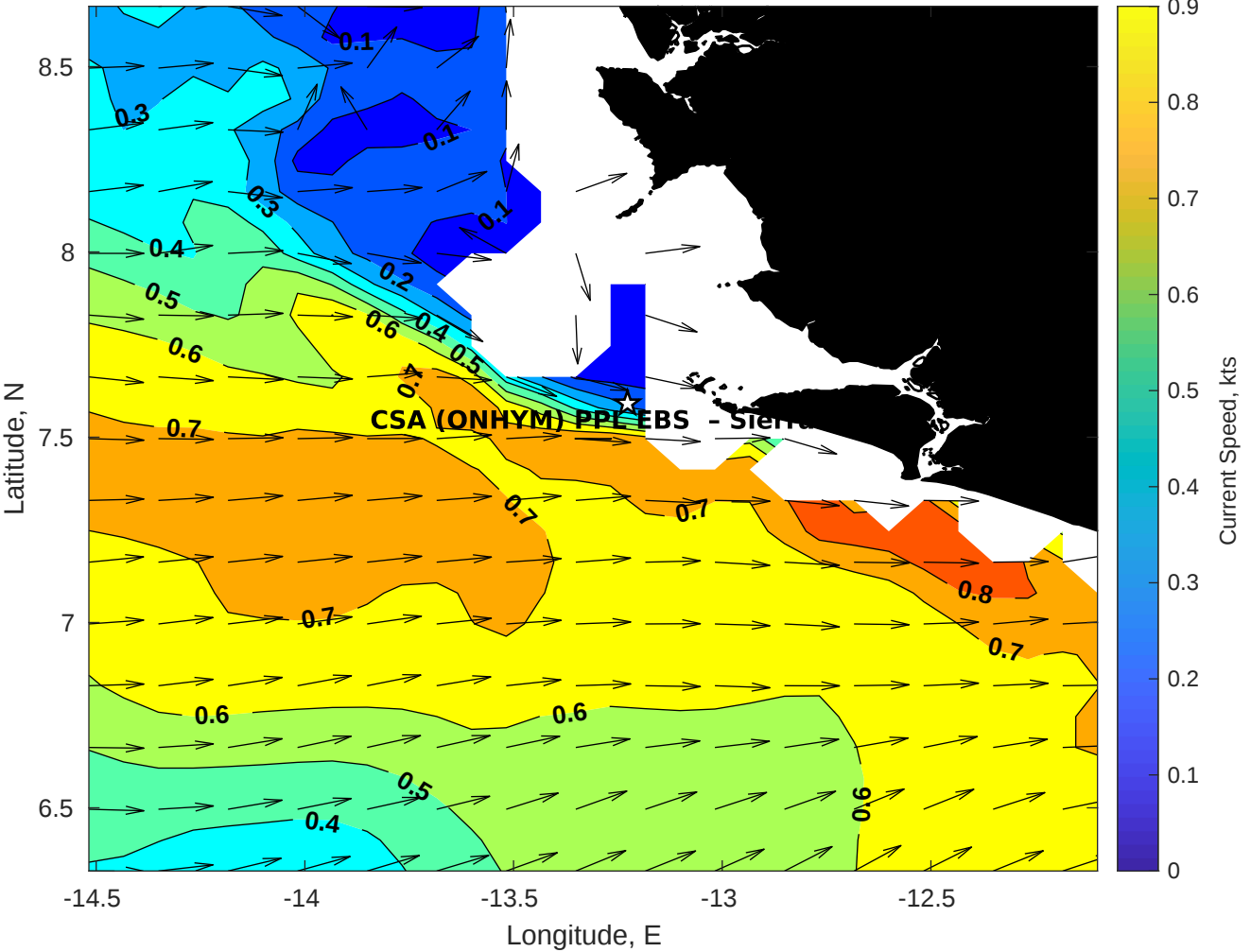
Surface Currents for CSA (ONHYM) PPL EBS - Sierra Leone at 21-Aug-2025 00:00:00
