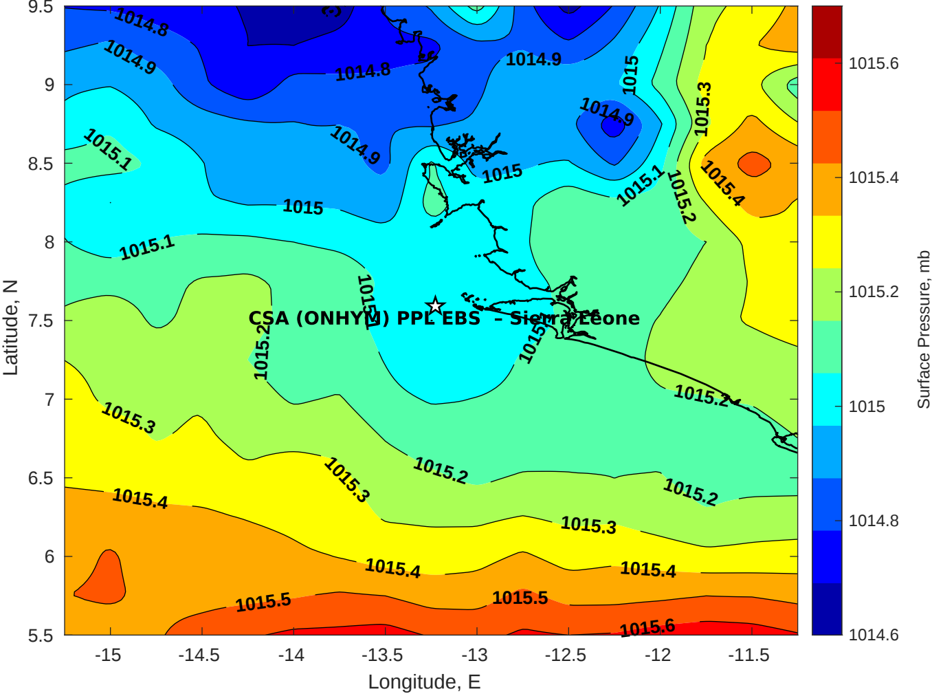
Surface Pressure (mb) for CSA (ONHYM) PPL EBS - Sierra Leone at 24-Aug-2025 00:00:00
