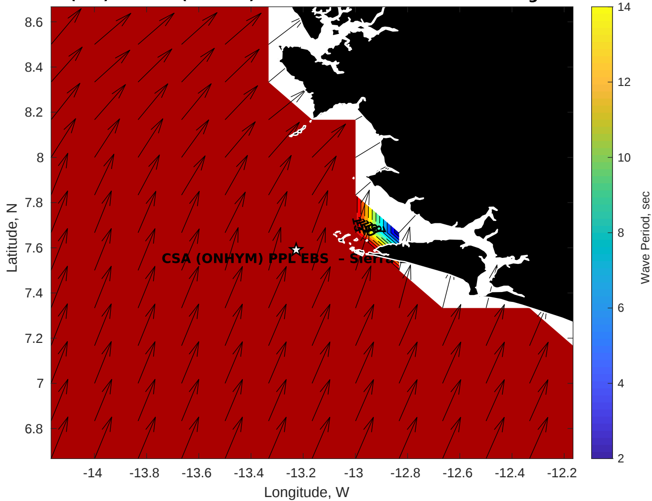
Wave Period (sec) for CSA (ONHYM) PPL EBS - Sierra Leone at 22-Aug-2025 09:00:00
