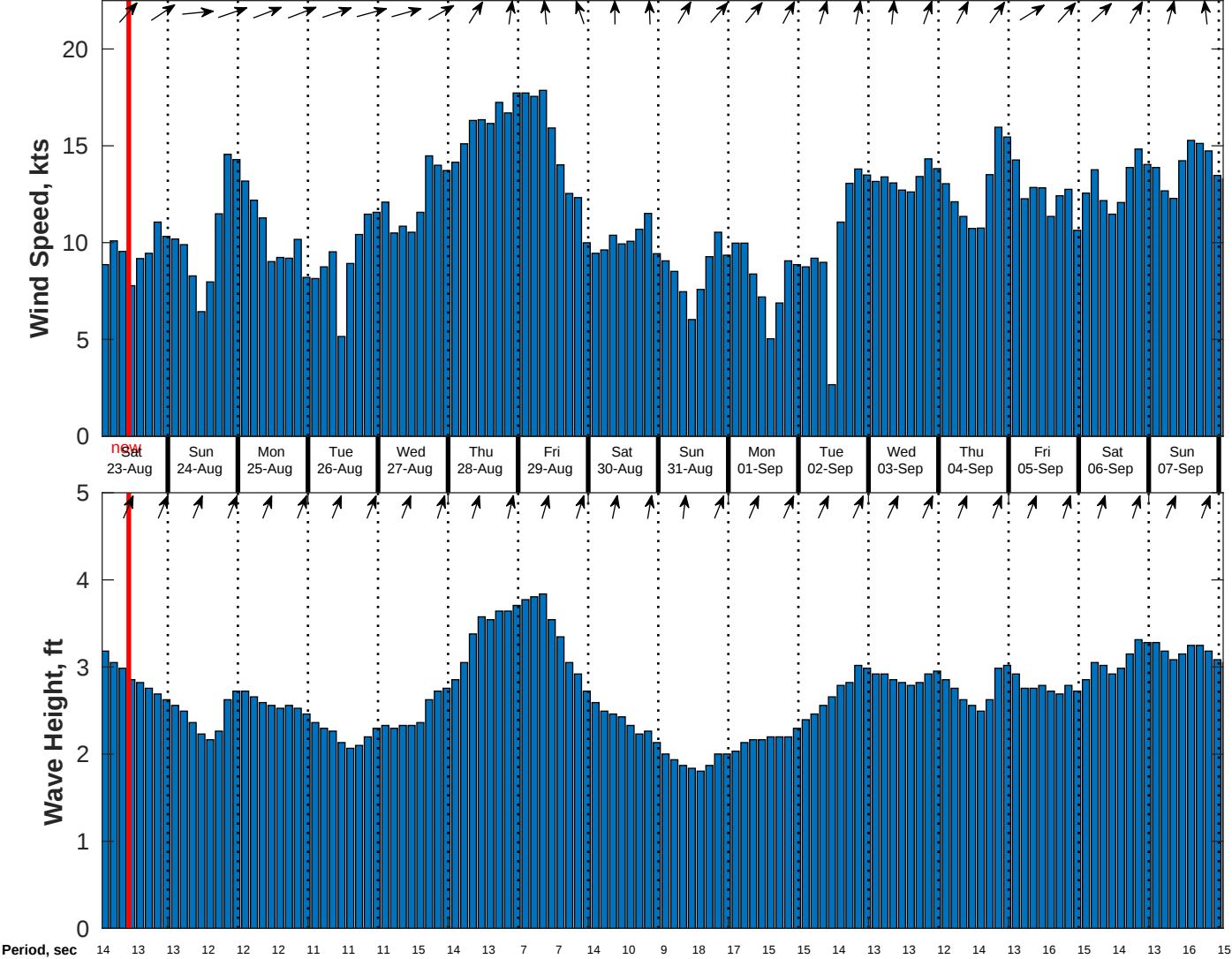
Wind & Wave Forecast for CSA (ONHYM) PPL EBS - Sierra Leone from 22-Aug-2025 01:00:00 to 07-Sep-2025 01:00:00
