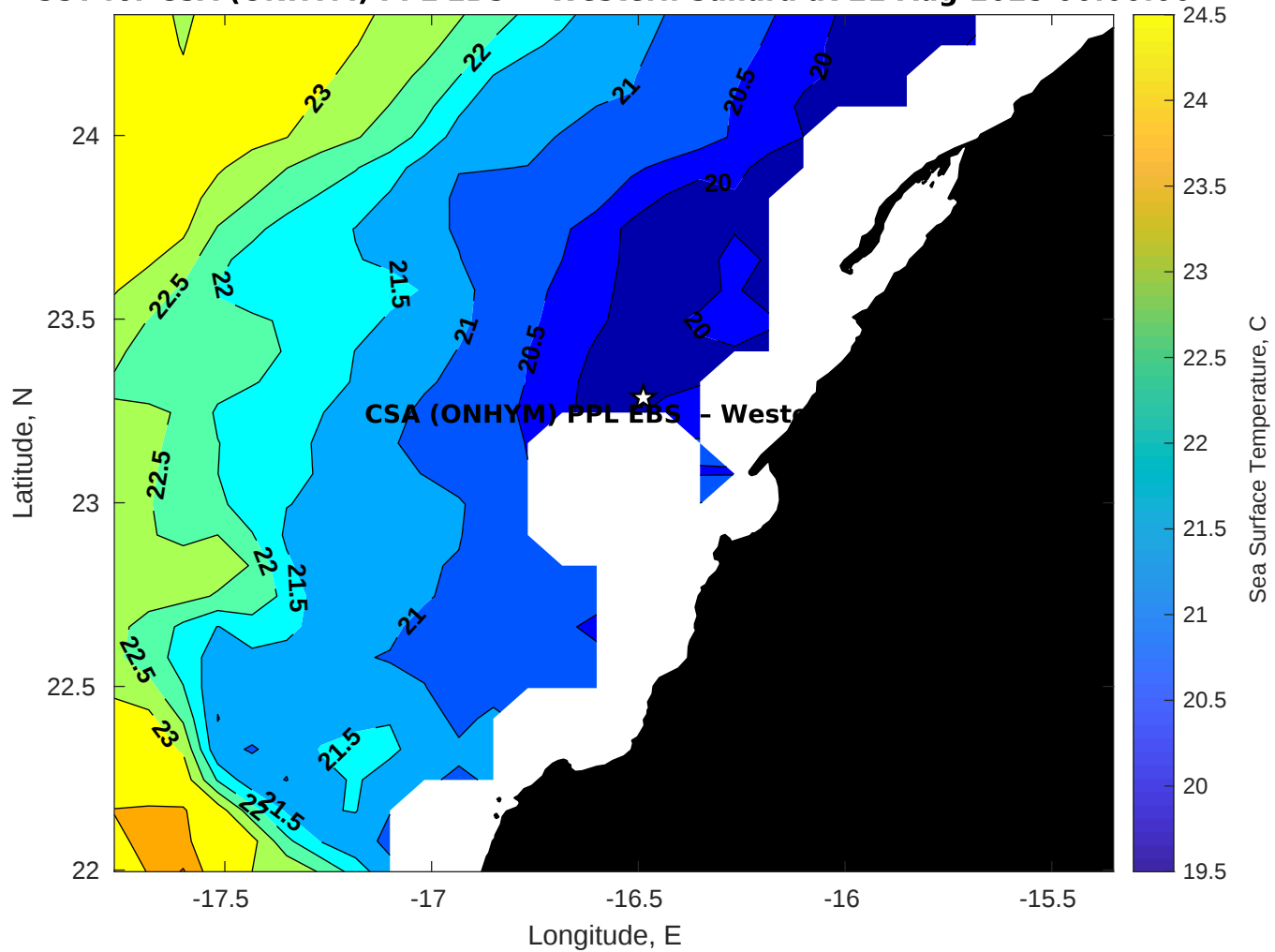
SST for CSA (ONHYM) PPL EBS - Western Sahara at 21-Aug-2025 00:00:00
