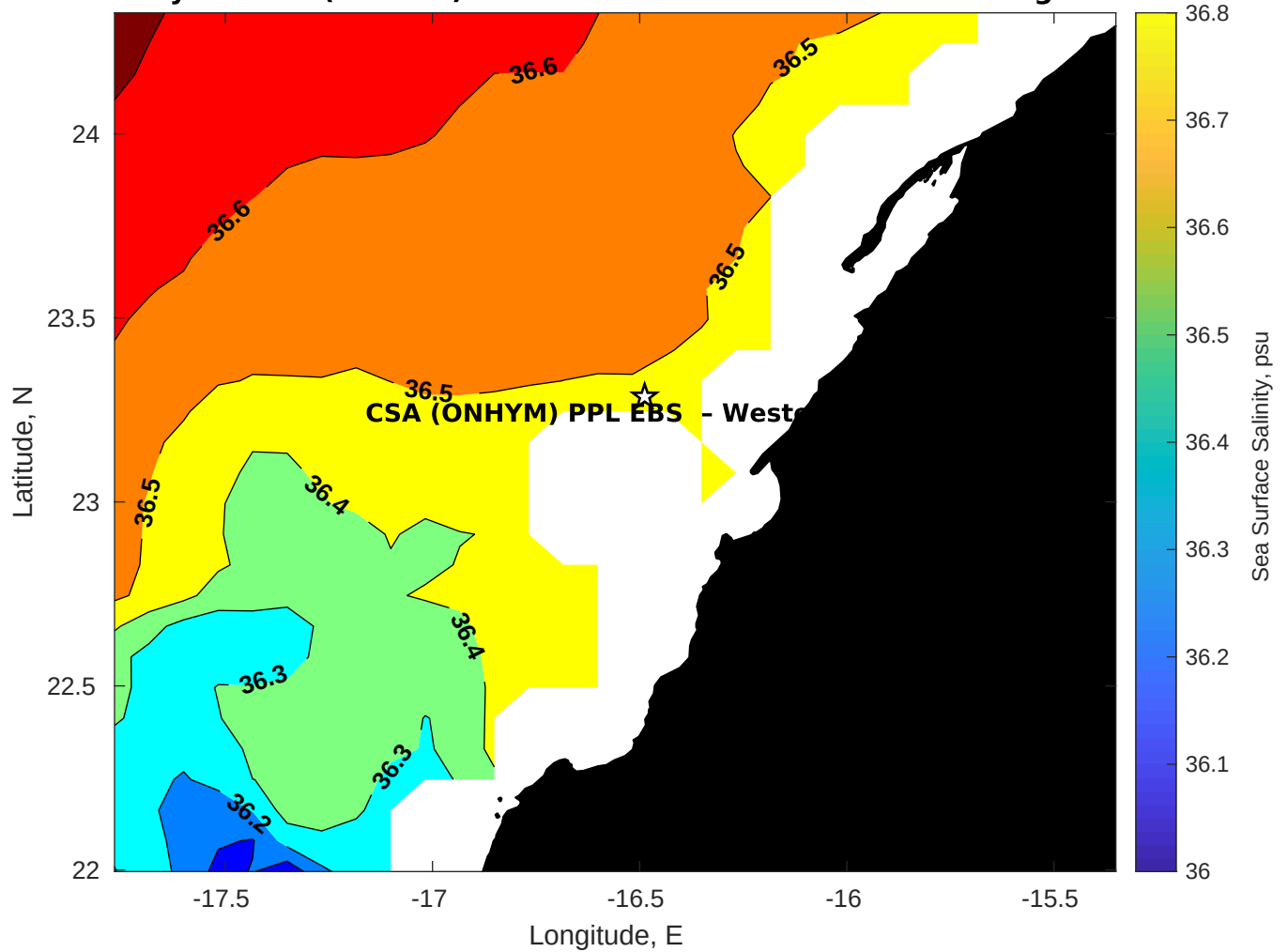
Surface Salinity for CSA (ONHYM) PPL EBS - Western Sahara at 21-Aug-2025 00:00:00
