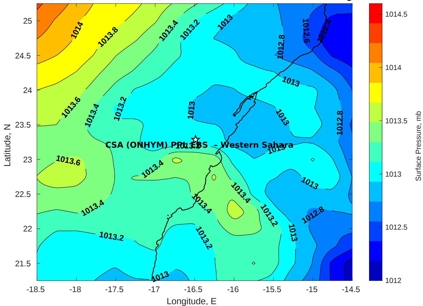
Surface Pressure (mb) for CSA (ONHYM) PPL EBS - Western Sahara at 22-Aug-2025 00:00:00
