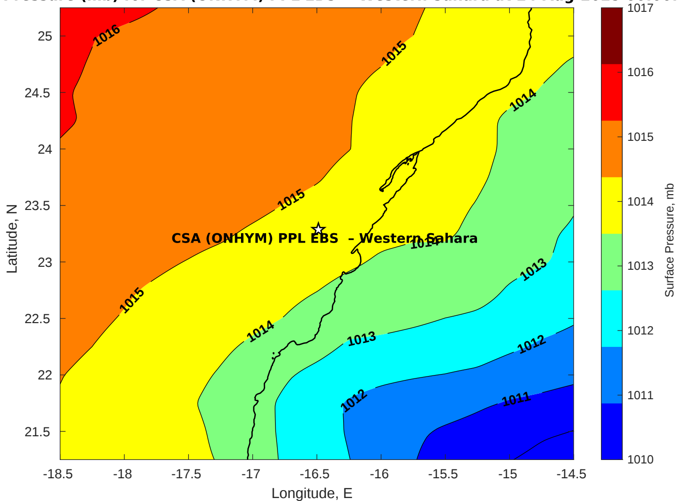
Surface Pressure (mb) for CSA (ONHYM) PPL EBS - Western Sahara at 24-Aug-2025 00:00:00
