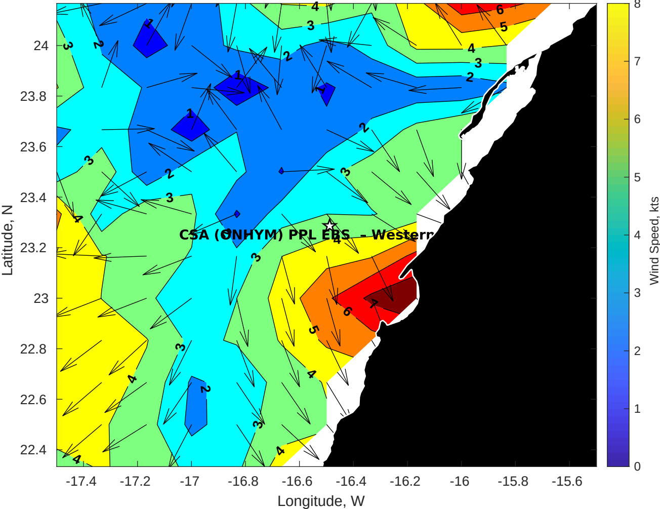
Winds (kts) for CSA (ONHYM) PPL EBS - Western Sahara at 22-Aug-2025 09:00:00
