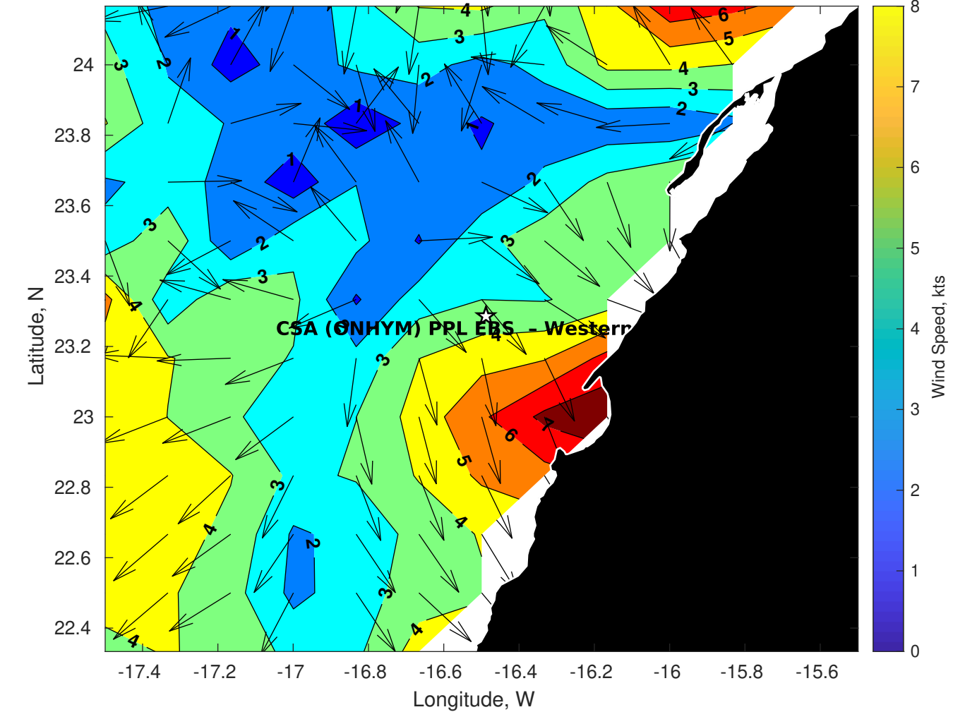
Winds (kts) for CSA (ONHYM) PPL EBS - Western Sahara at 22-Aug-2025 09:00:00
