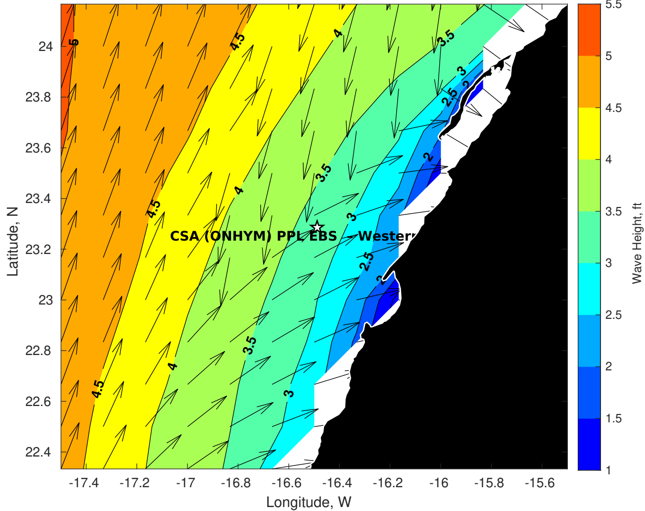
Wave Height (ft) for CSA (ONHYM) PPL EBS - Western Sahara at 22-Aug-2025 09:00:00
