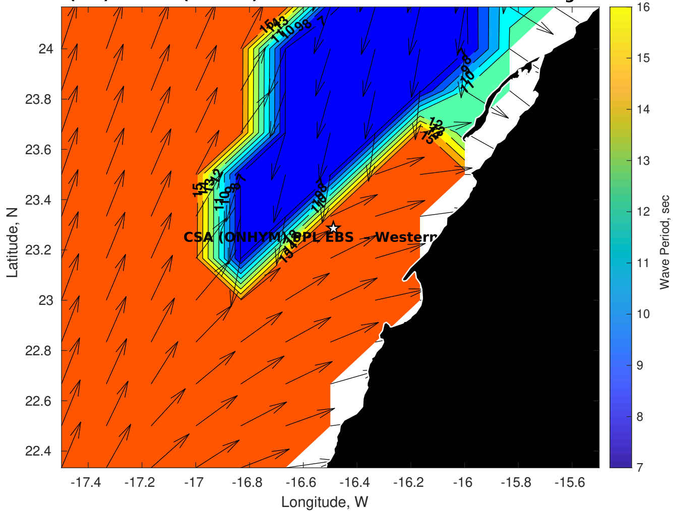
Wave Period (sec) for CSA (ONHYM) PPL EBS - Western Sahara at 22-Aug-2025 09:00:00
