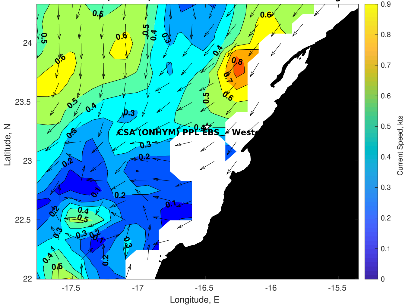
Surface Currents for CSA (ONHYM) PPL EBS - Western Sahara at 21-Aug-2025 00:00:00
