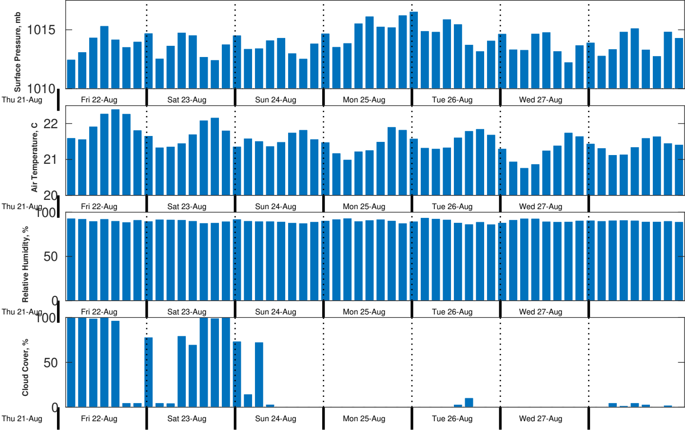
Met Forecast for CSA (ONHYM) PPL EBS - Western Sahara from 22-Aug-2025 00:00:00 to 29-Aug-2025 00:00:00
