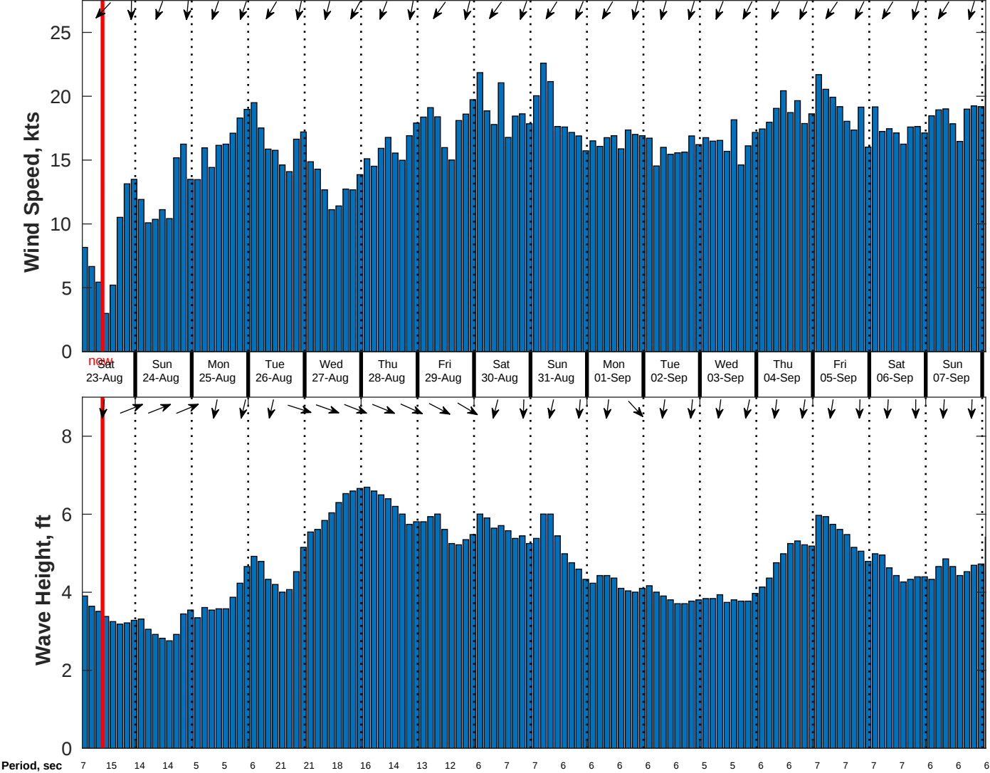
Wind & Wave Forecast for CSA (ONHYM) PPL EBS - Western Sahara from 22-Aug-2025 01:00:00 to 07-Sep-2025 01:00:00
