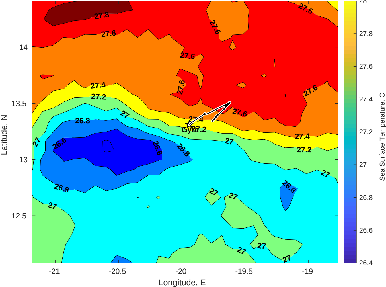
SST for Gyre at 21-Aug-2025 00:00:00
