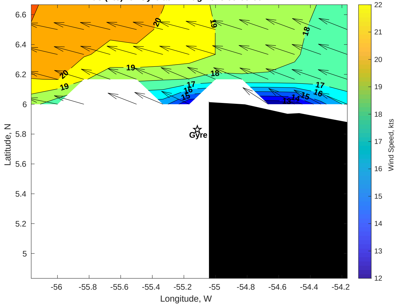
Winds (kts) for Gyre at 22-Aug-2025 09:00:00
