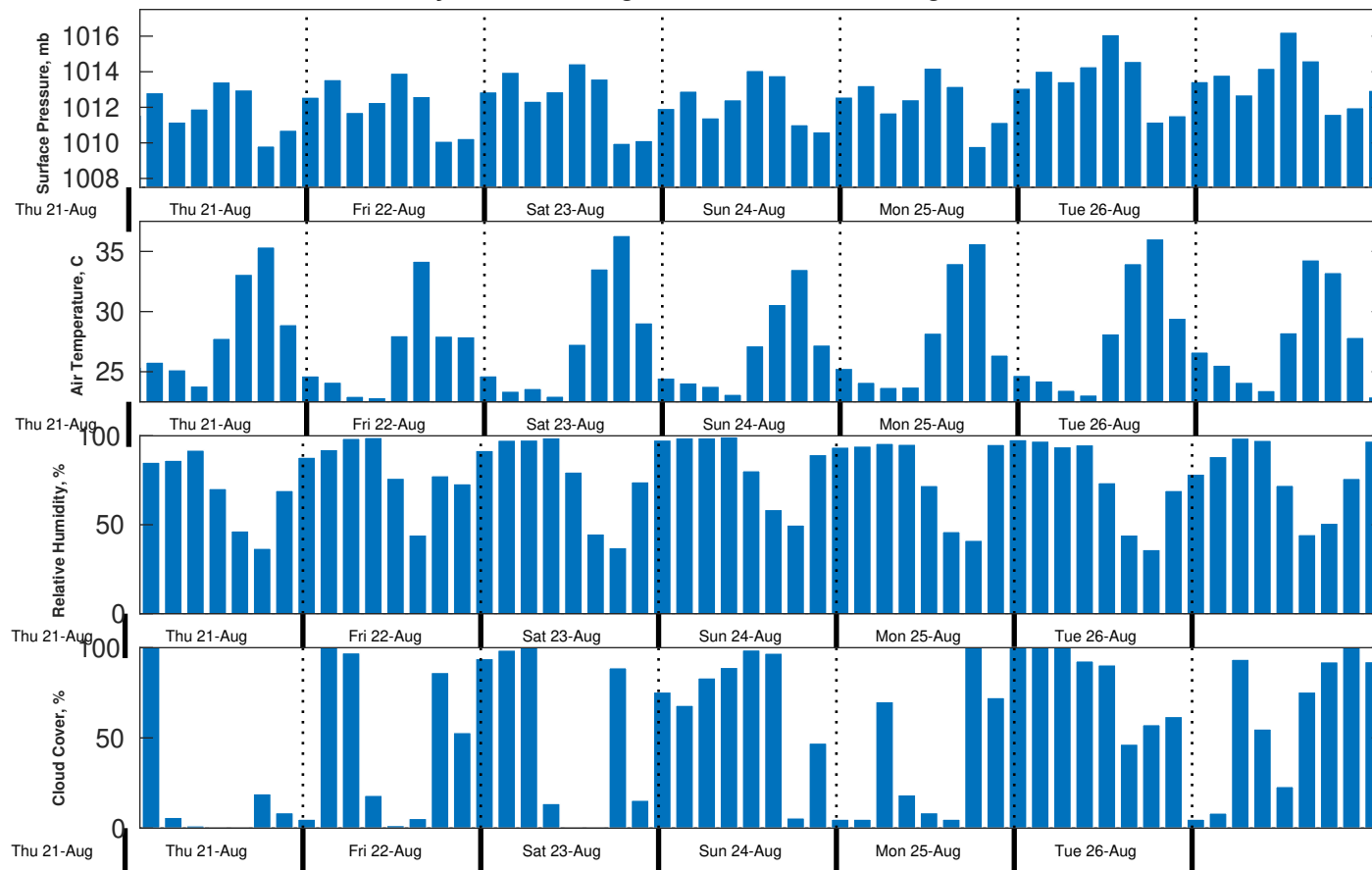
Met Forecast for Gyre from 21-Aug-2025 20:00:00 to 28-Aug-2025 20:00:00
